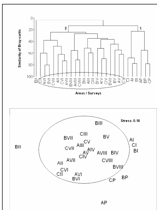
Figure 6. Cluster analysis (UPGMA) and MDS ordination (Bray-Curtis similarity coefficient), included the nine surveys in the three study areas (A = Orion reef, B and C = controls, P = pre-monitoring and I to VIII = monitoring surveys), considering the 23 species with > 10 individuals in at least one of the areas.
