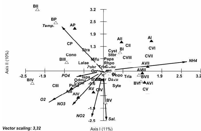
Figure 7. Canonical correspondence analysis. Factorial diagram showing the most abundant species in biomass and most frequent (65%) in the surveys (P = pre-monitoring and I to VIII = post-monitoring). Environmental parameters: temperature, salinity, dissolved oxygen, nitrite, nitrate, ammonia and phosphate on the Orion reef (area A) and control areas B and C. Species code on Table 2.
