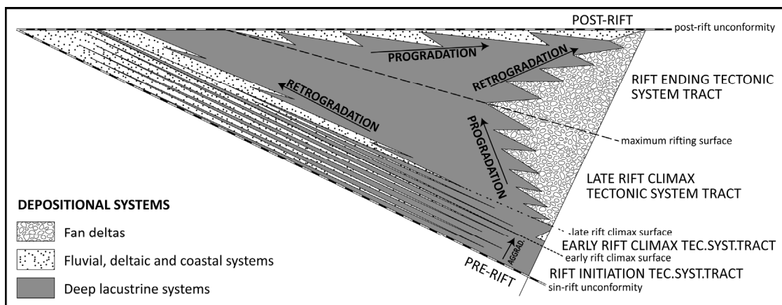
Figure 8: Idealized model of Tectonic System Tracts, showing the depositional systems and stacking patterns in relation to the region of the half-graben (controlled by axial/marginal drainage at the flexural margin, or by the border fault drainage). The surfaces that bound the tectonic system tract are also indicated.
