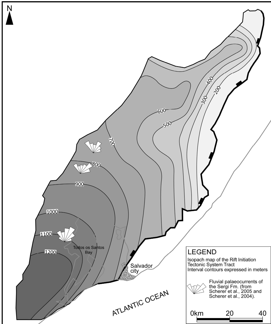
Figure 11: Isopach map of the Rift Initiation Tectonic System Tract of the Recôncavo Basin, comprising the Aliança and Sergi Fms. (Brotas Group). Adapted from Netto et al. (1982).
