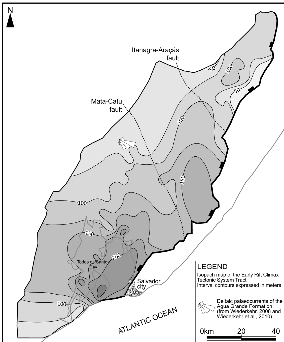
Figure 12: Isopach map of the Early Rift Climax Tectonic System Tract of the Recôncavo Basin, comprising the Itaparica and Água Grande Fms. and the Tauá Mb. of the Candeias Fm. Adapted from Figueredo et al. (1994).
