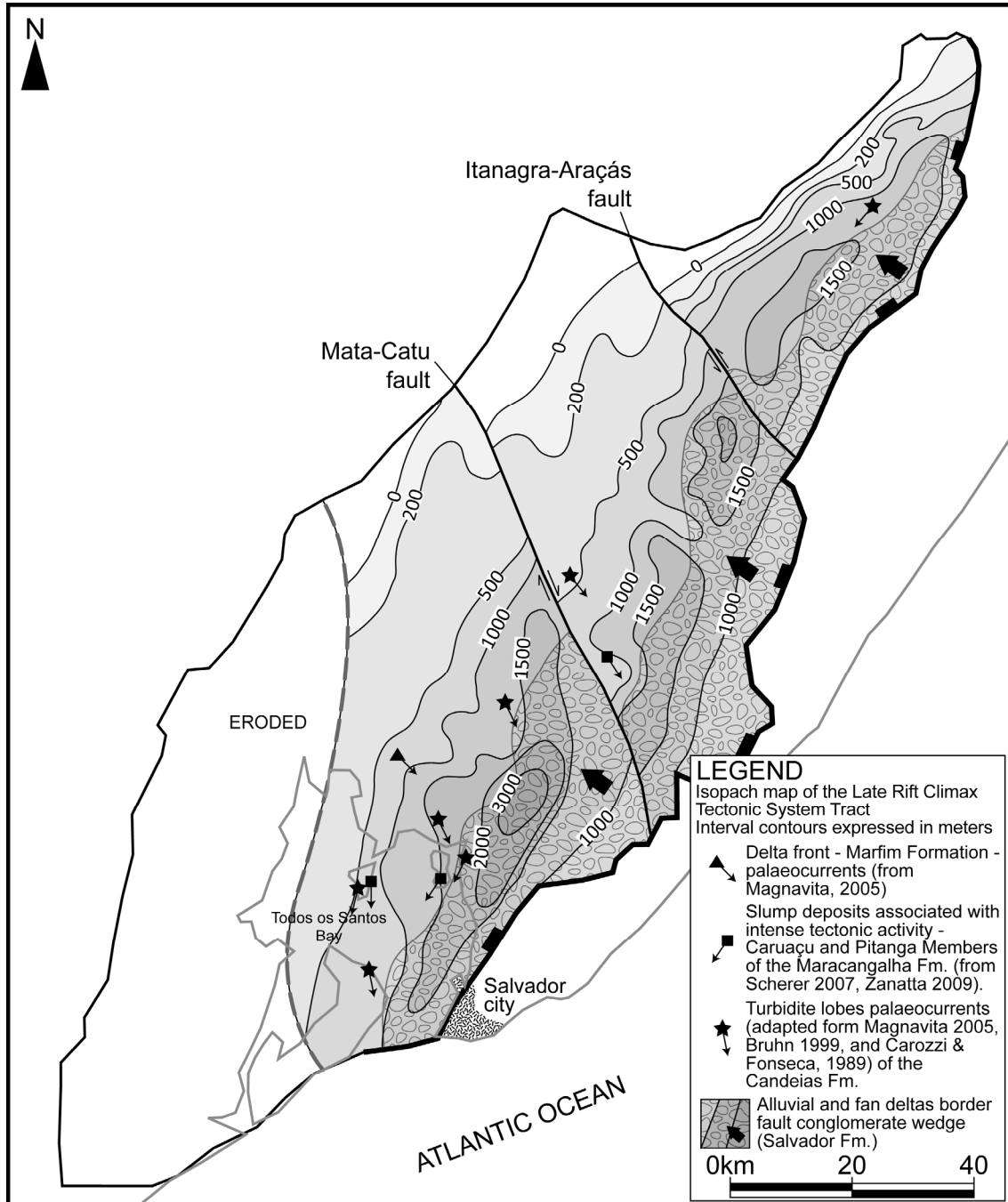
Figure 13: Isopach map of the Late Rift Climax Tectonic System Tract of the Recôncavo Basin, comprising the Gomo Mb. of the Candeias Fm., and the basal part of the Maracangalha Fm. (including the Caruaçu and Pitanga Mbs.). Adapted from Figueredo et al. (1994).
