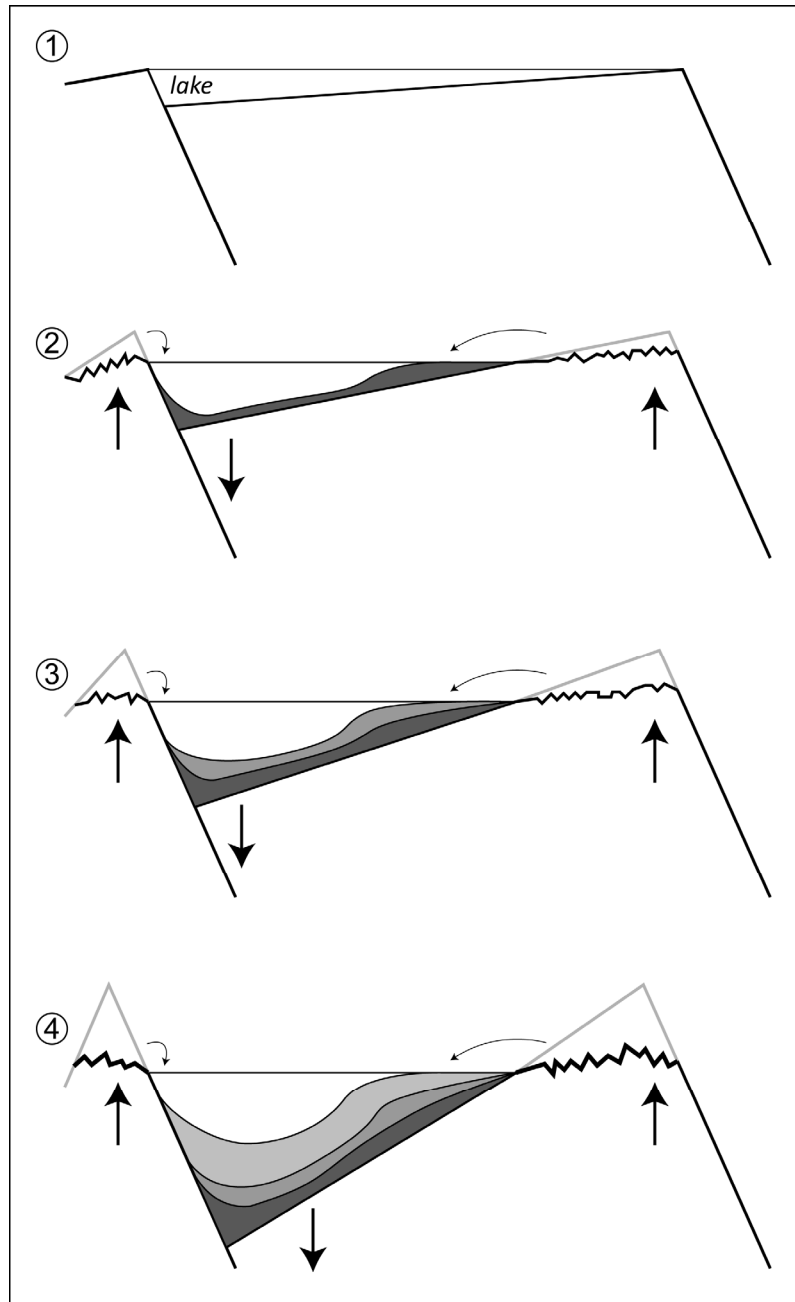
Figure 2: model of evolution of a half-graben related to a tectonic pulse, responsible for the creation of accommodation on the hangingwall at the same time of erosion on the footwals , what consequently generates a depositional package genetically correlated laterally to an erosion surface.
