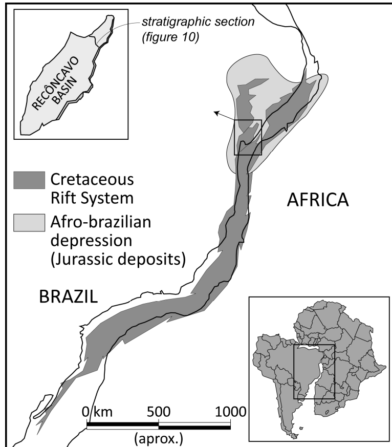
Figure 9: Simplified map of the Afro-Brazilian Depression, showing its spatial relationship with the Atlantic Cretaceous Rift System. The Recôncavo Basin is an aborted arm of the rift system located at the northeastern region of Brazil, and shows a half-graben structure entirely preserved, unlike the marginal Atlantic basins, which due to the rupture show a fragmented rift structure. Modified from Figueredo et al. (1994).
