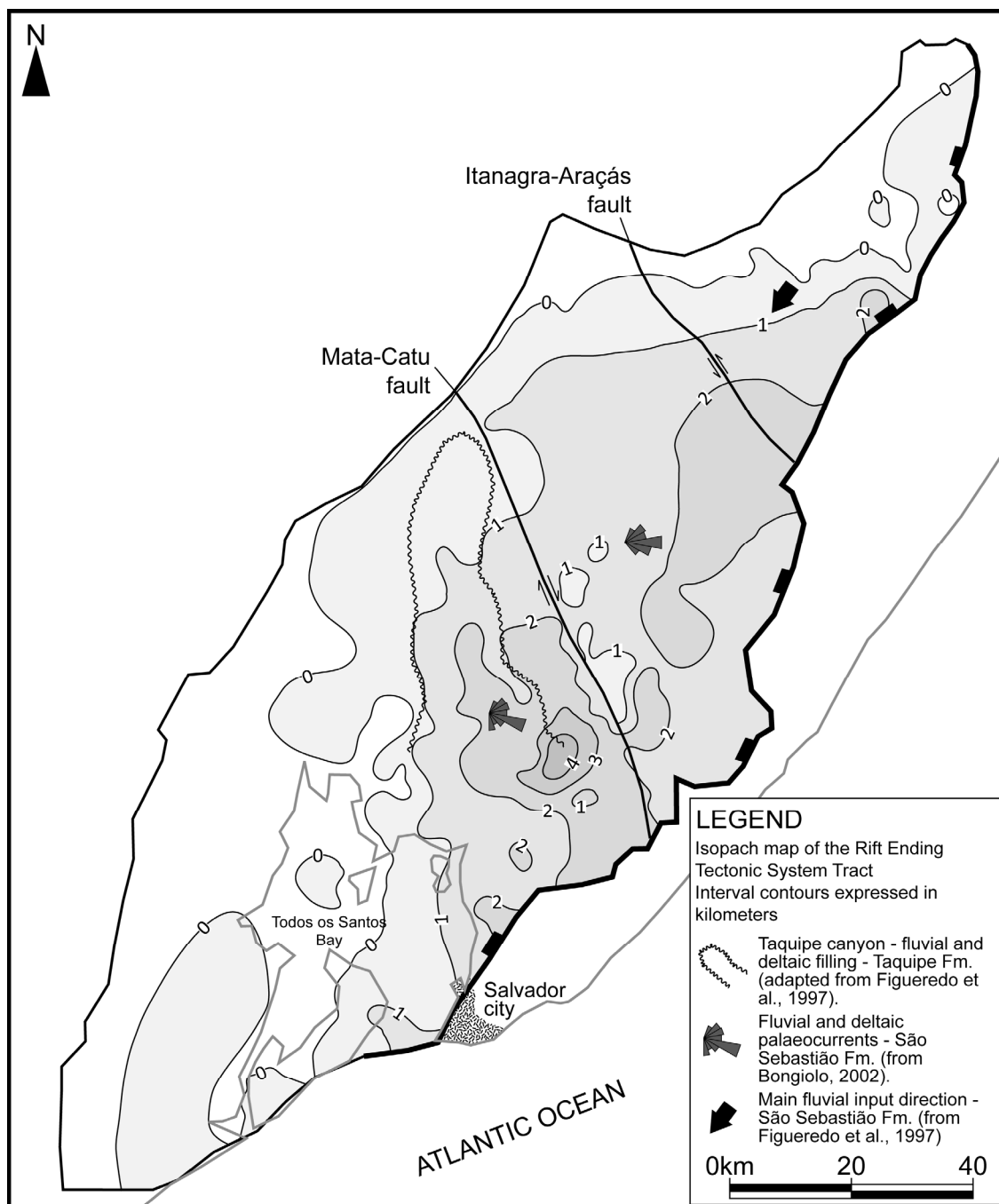
Figure 14: Isopach map of the Rift Ending Tectonic System Tract of the Recôncavo Basin, comprising the top part of the Maracangalha Fm. (not including Caruaçu and Pitanga Mbs.), Marfim, Pojuca, Taquipe and São Sebastião Fms. Adapted from Figueredo et al. (1994).
