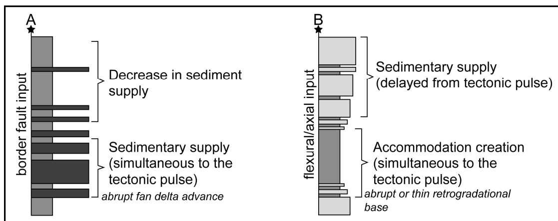
Figure 5: The result of the delay is a progradational to retrogradational facies succession response to the border fault drainage (facies succession A), whereas at the flexural margin site (facies succession B) a retrogradational to progradational pattern occurs, which indicates that sedimentation during the tectonic pulse is represented by fine sediments of deep lacustrine systems (low supply situation), overlain by coarsening-upward sediments of marginal lake and continental systems (high supply – delayed – condition).
