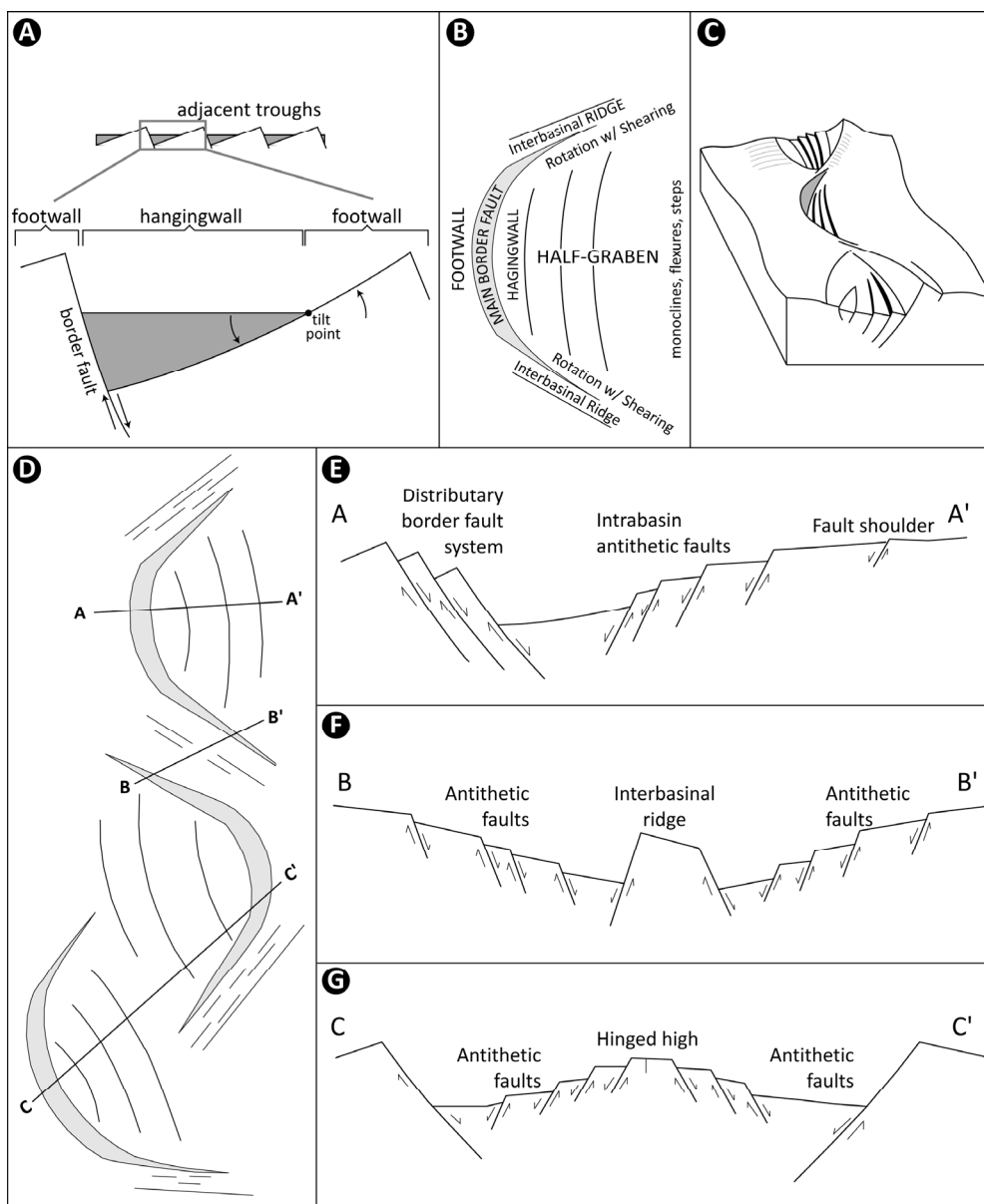
Figure 1, A: Individual half-graben and its internal compartmentation in footwal (uplifted portion), and hangingwall (subsided portion). The tilt point controls the transition footwal/hangingwall at the flexural margin. B: overview of a unique half-graben structure, with lateral termination of the border fault and its internal structures (modified from Rosendhal et al. , 1986). C: 3D view of the half-graben as pictured in frame B (modified from Rosendhal et al. , 1986). D: map of the half-graben composite interaction as showed in the profiles of frames E, F and G. E,F,G: Profiles of half-grabens and its interactions and internal structures, as showed in the map of frame D (modified from Rosendhal et al. , 1986).
