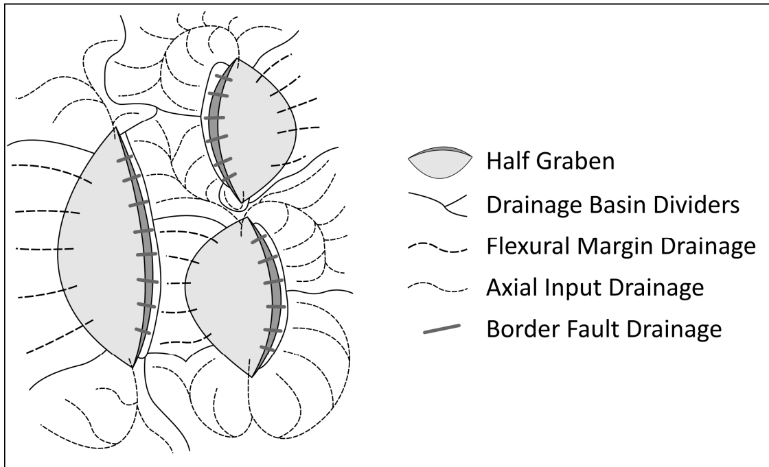
Figure 3: Compartmentation of the half-graben drainage system in three types: flexural margin, axial input and border fault drainages. The topographic highs are the drainage basin dividers.
