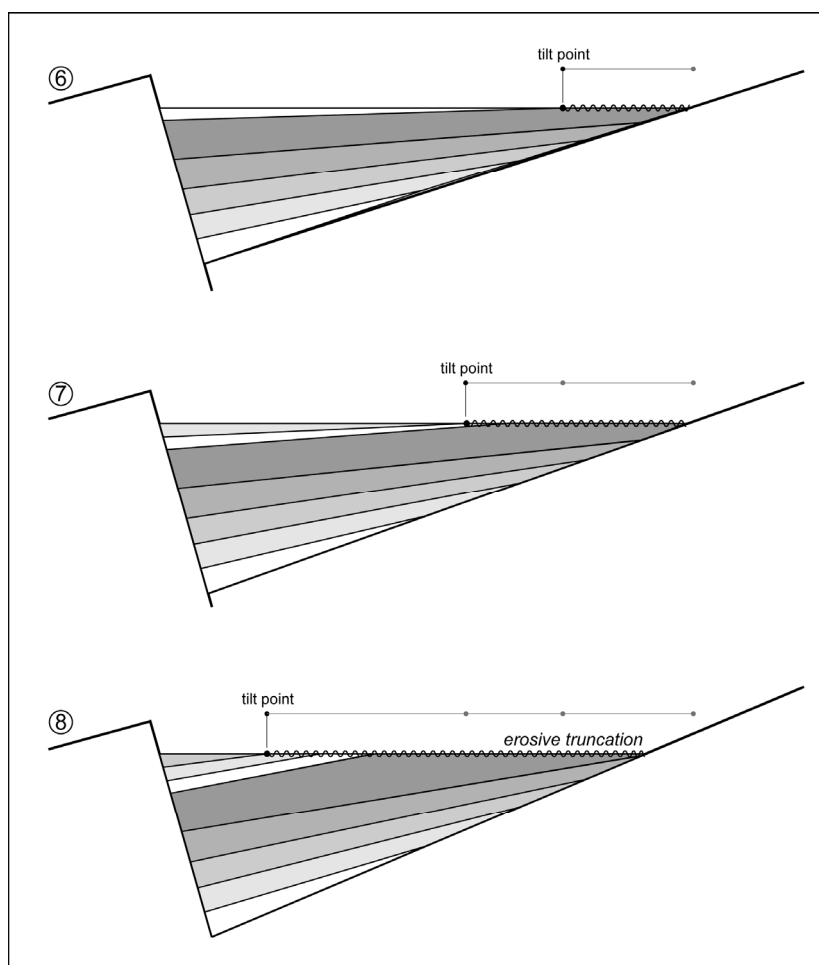
Figure 7: Migration of the tilt point basinward during accommodation creation. It generates a retreat of the half-graben area and erosive truncations at the top of older units.
