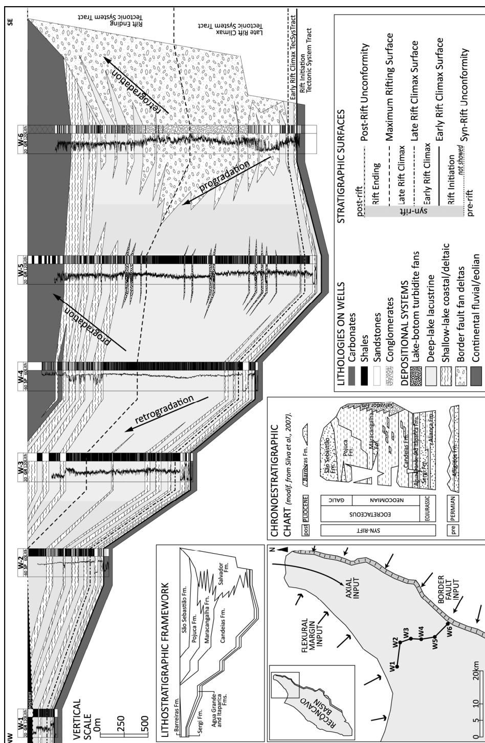
Figure 10: Stratigraphic section in the northern compartment of the Recôncavo Basin, perpendicular to the half-graben (dip-oriented), as showed in the basic map. The main lithostratigraphic units are showed in the chronostratigraphic chart and the schematic synthesis of the lithostratigraphic framework. The section is showed on true vertical depth from the actual terrain surface. The stratigraphic framework of the section shows the tectonic system tracts and their bounding surfaces, the interpreted depositional systems and the lithologic data of the wells. Wells W1 to W5 show the flexural margin stacking pattern, whereas well W6 shows the border fault pattern.
