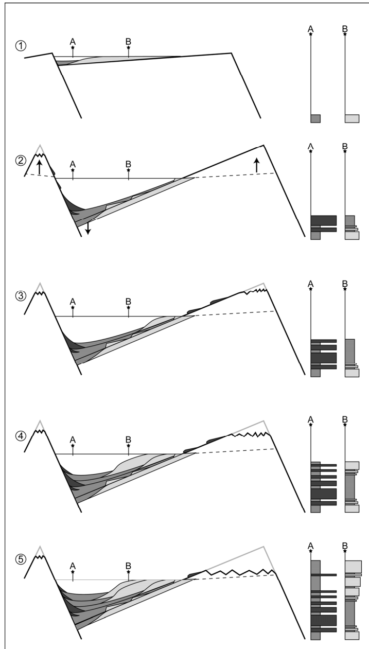
Figure 4: model of evolution of a half-graben related to an instantaneous tectonic pulse. The rapid creation of accommodation (from time 1 to 2) generates an intense retrogradational pattern at the flexural margin (well B), whereas near at the border fault, fan delta progradation occurs. Retrogradation at the flexural margin is related to the low sediment supply at this moment, due to the rearrangement of drainage pattern and the time necessary for erosion and transport (time 2 and 3). After the pulse, the drainage is established and erosion of the flexural margin begins. The sedimentary supply surpasses accommodation, generating a progradational pattern at the flexural margin. At the same time, ceasing of the tectonic activity generates the retreat of fan deltas related to the border fault, generating a retrogradation at this site (time 4 and 5).
