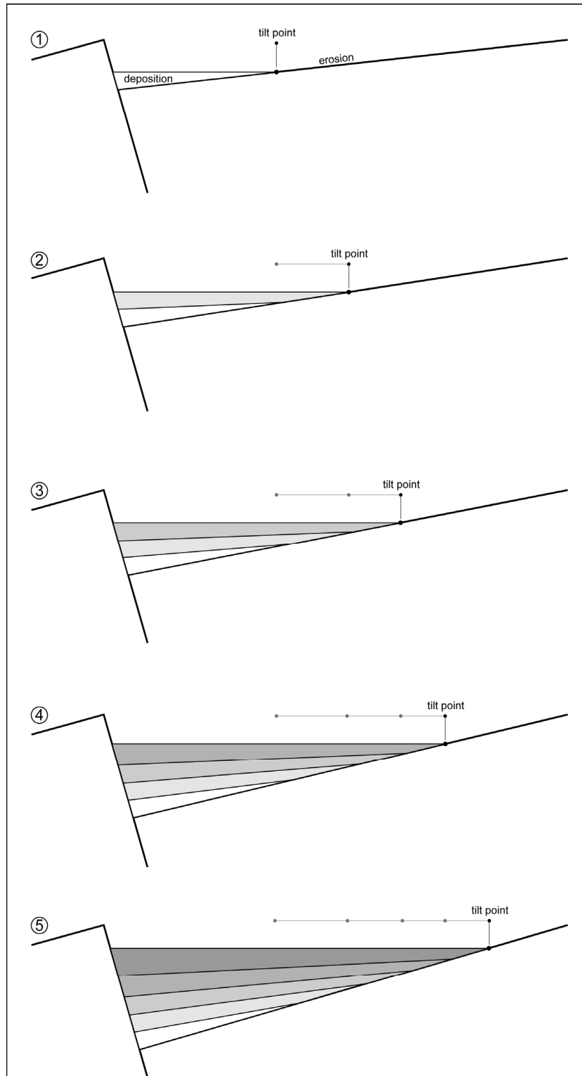
Figure 6: Migration of the tilt point landward during accommodation creation. It generates an expansion of the half-graben, successive onlaps at the base and rearrangement of the drainage pattern.
