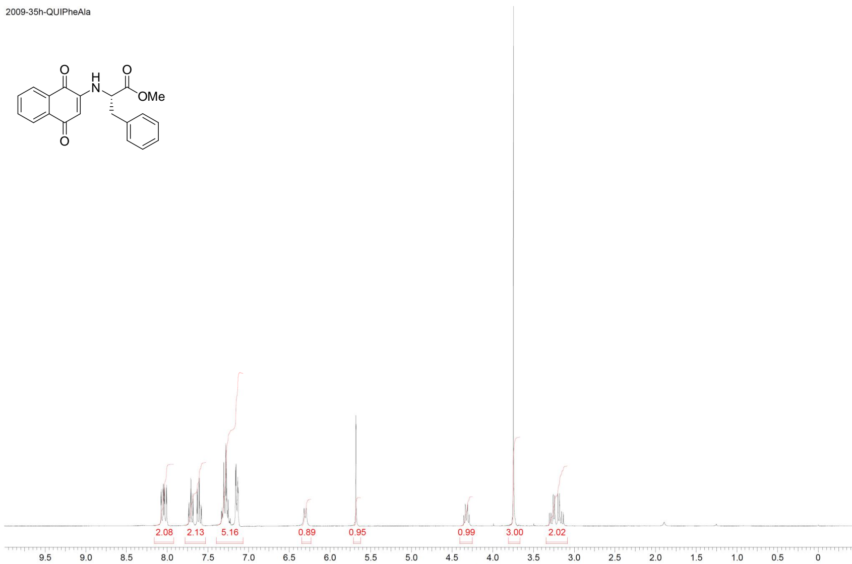
Espectro E – 11.2 - (RMN ^1\text{H} , 300 MHz, \text{CDCl}_3 ) – Aminonaftoquinona 85j
