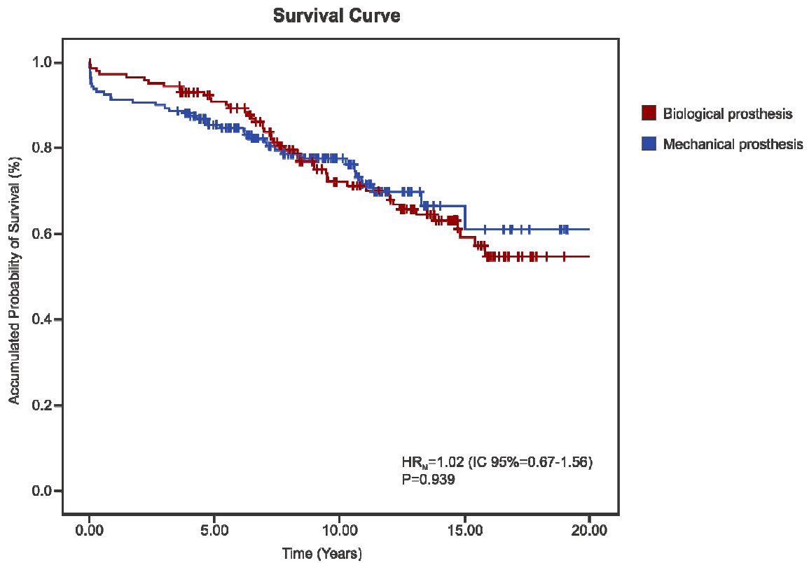
Figure 1 - Kaplan-Meier Curve to assess probability of survival.
