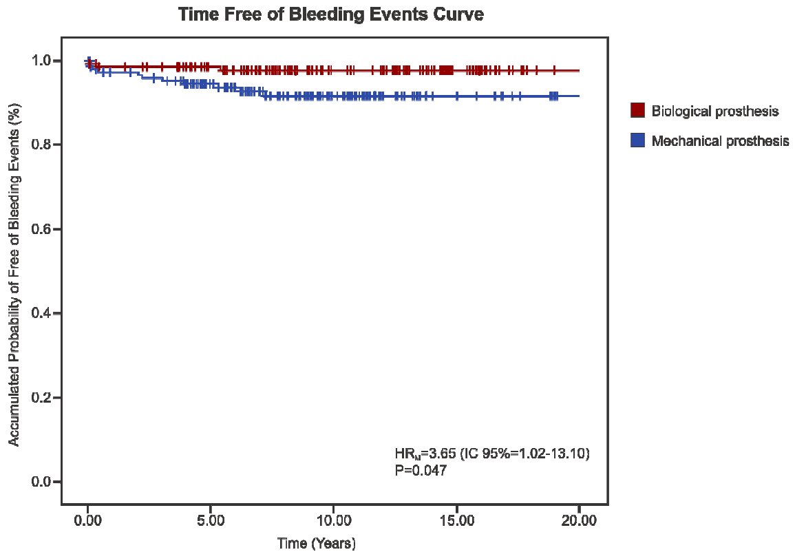
Figure 3 - Kaplan-Meier curve to assess time free of bleeding events.
