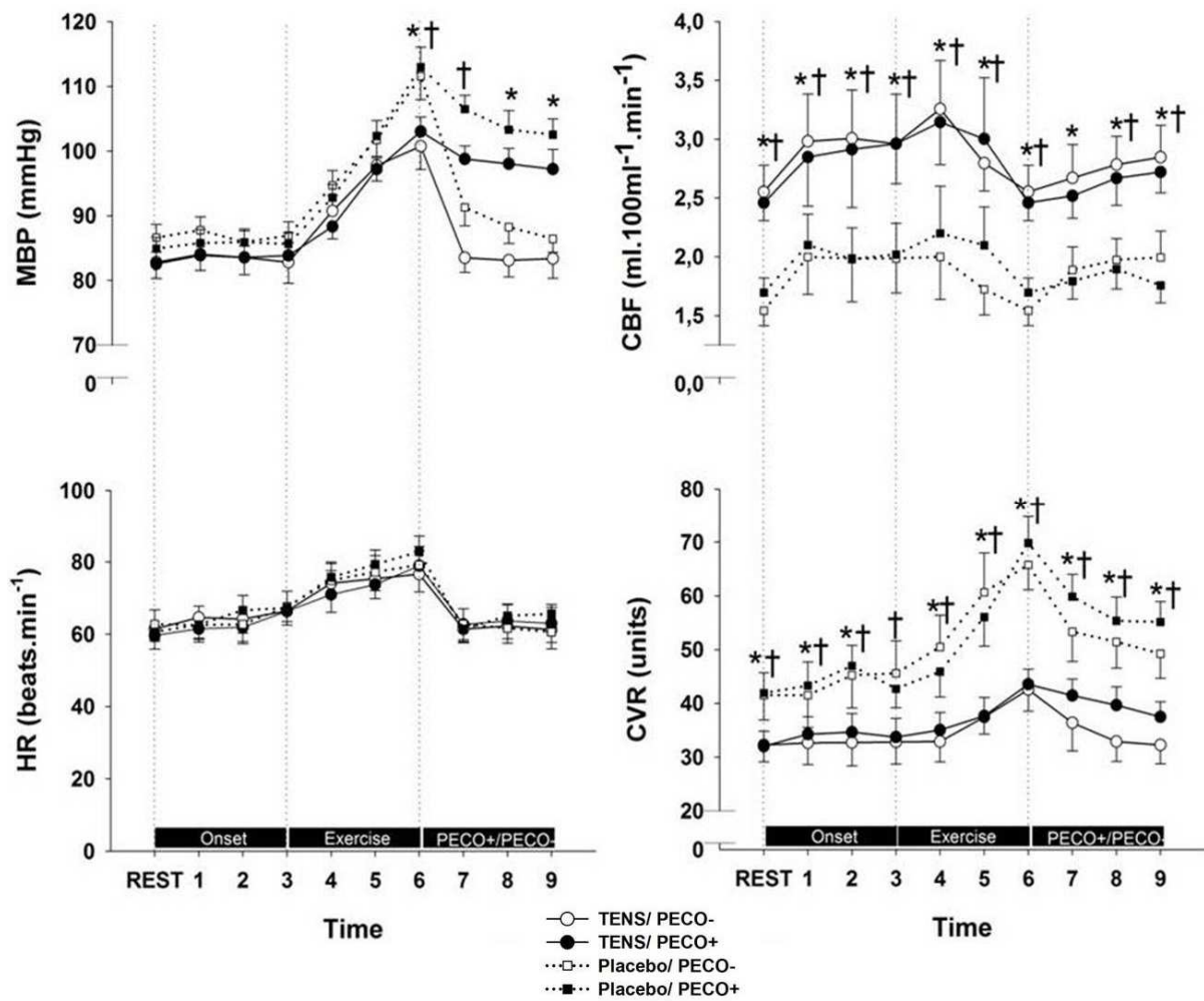
Fig. 1 Mean blood pressure (MBP), heart rate (HR), calf blood flow (CBF), and calf vascular resistance (CVR) in values absolute during static handgrip exercise, postexercise circulatory occlusion (PECO+) or without occlusion (PECO-) periods.
