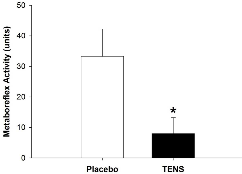
Fig. 2 Estimated muscle metaboreflex control of calf vascular resistance (CVR), obtained by the subtraction of the area under the curve in circulatory occlusion period (PECO+) from control period (PECO-) during TENS and Placebo situation.
