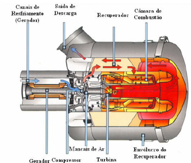
FIGURA 3.18 – Interior da Turbina Capstone.
