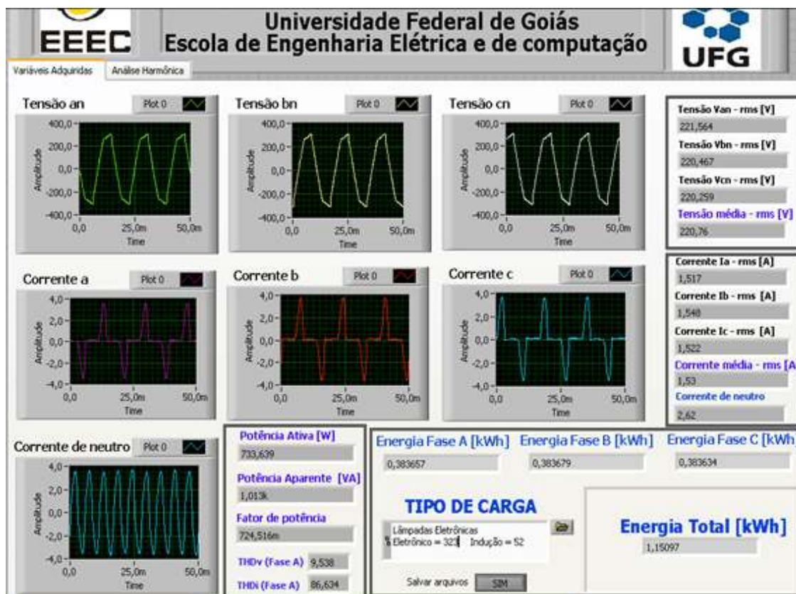
Fig. 5-1 – Painel Frontal 1 – LabVIEW.
