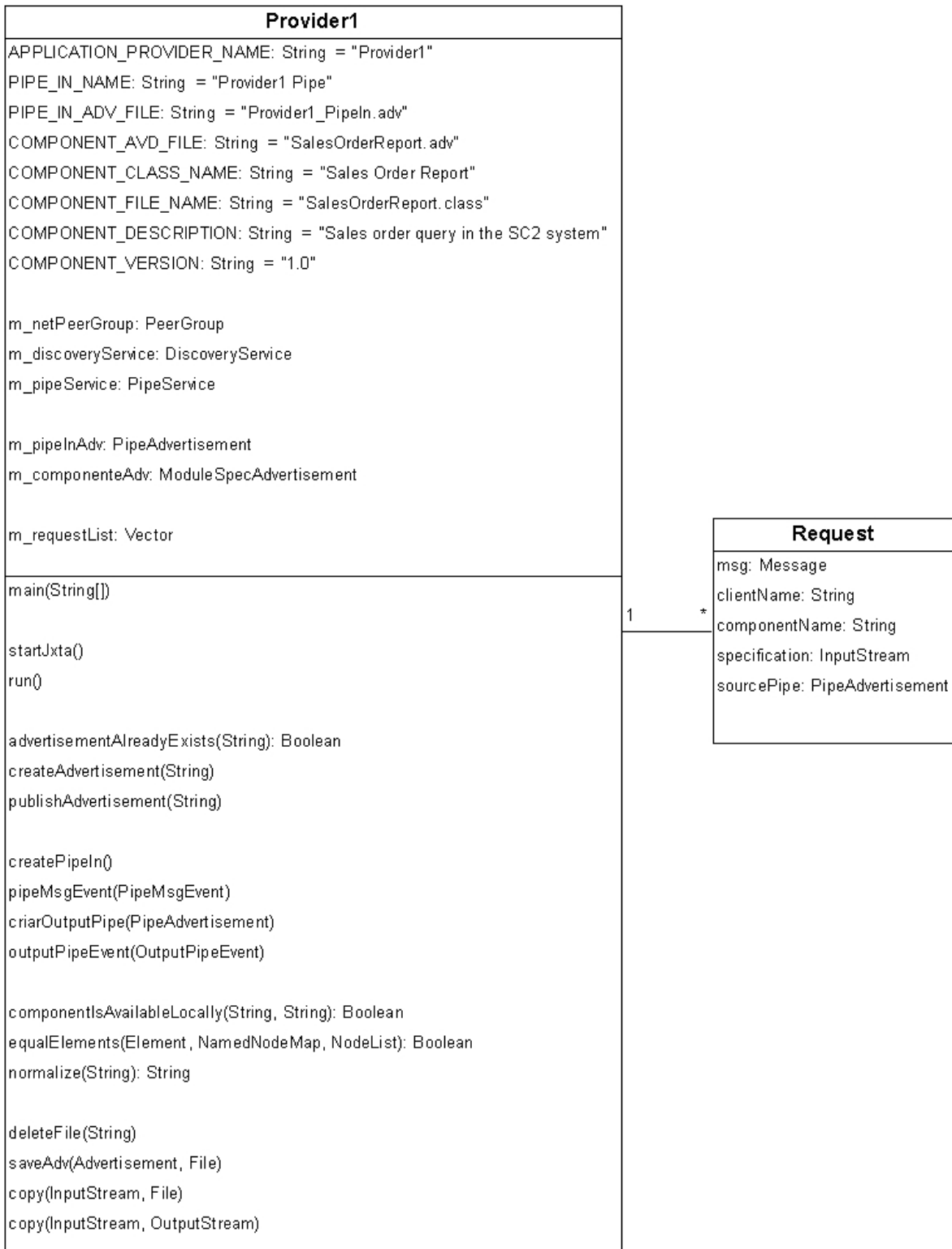
Figura 4.8 – Diagrama de Classes – PA
