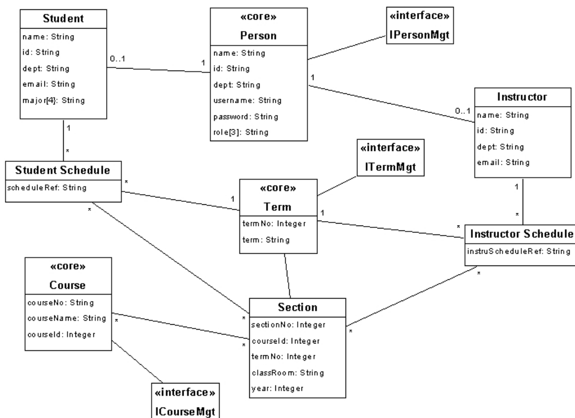
Figura 2.5 – Interface Responsibility Diagram (Liu et al., 2002)
