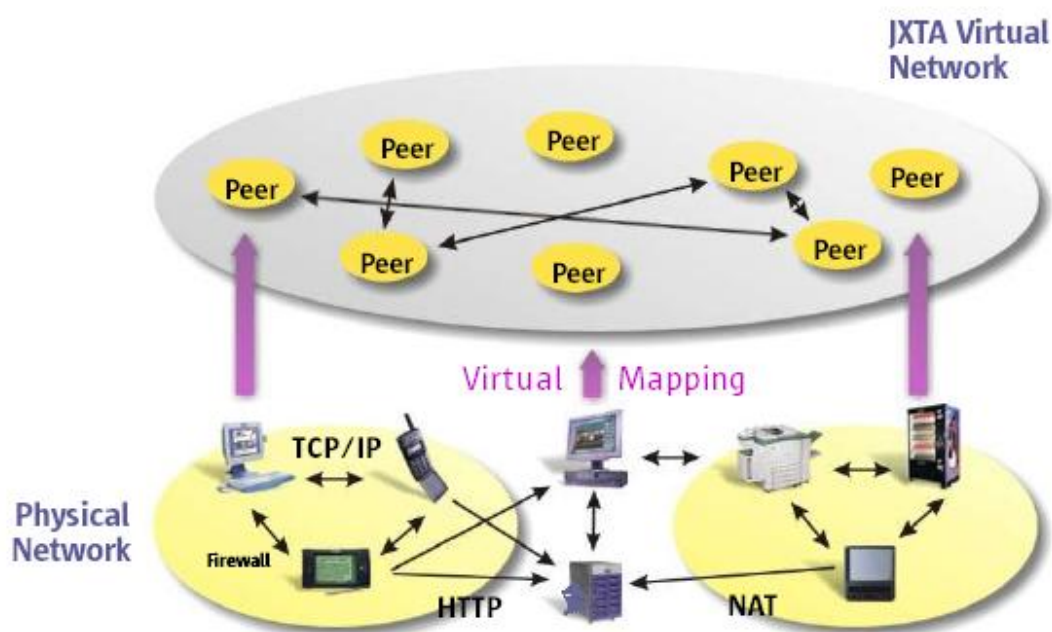
Figura 2.13 – Rede Virtual JXTA (JXTA, 2004b)
