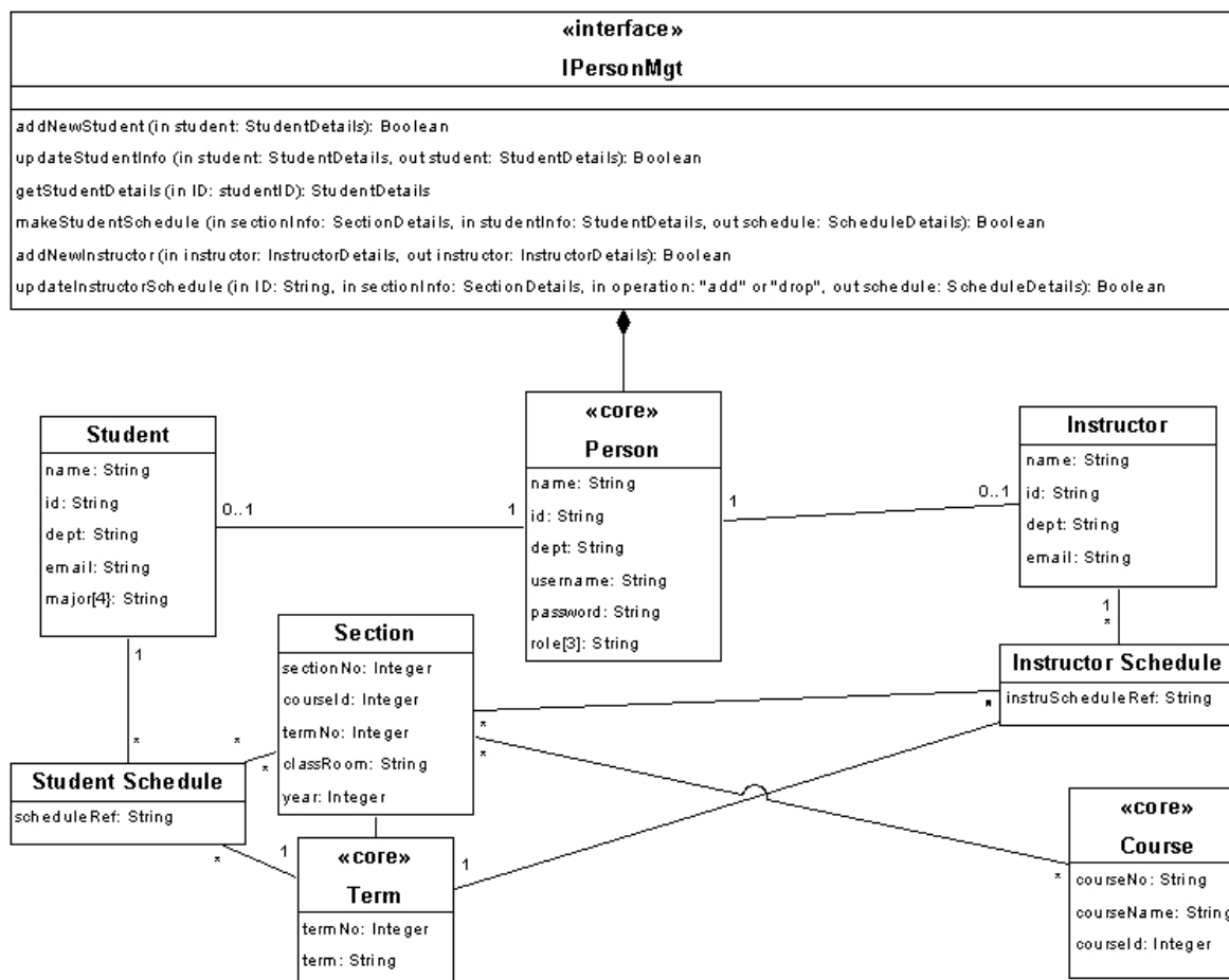
Figura 2.6 – Interface Information Model para a Interface IPersonMgt (Liu et al., 2002)
