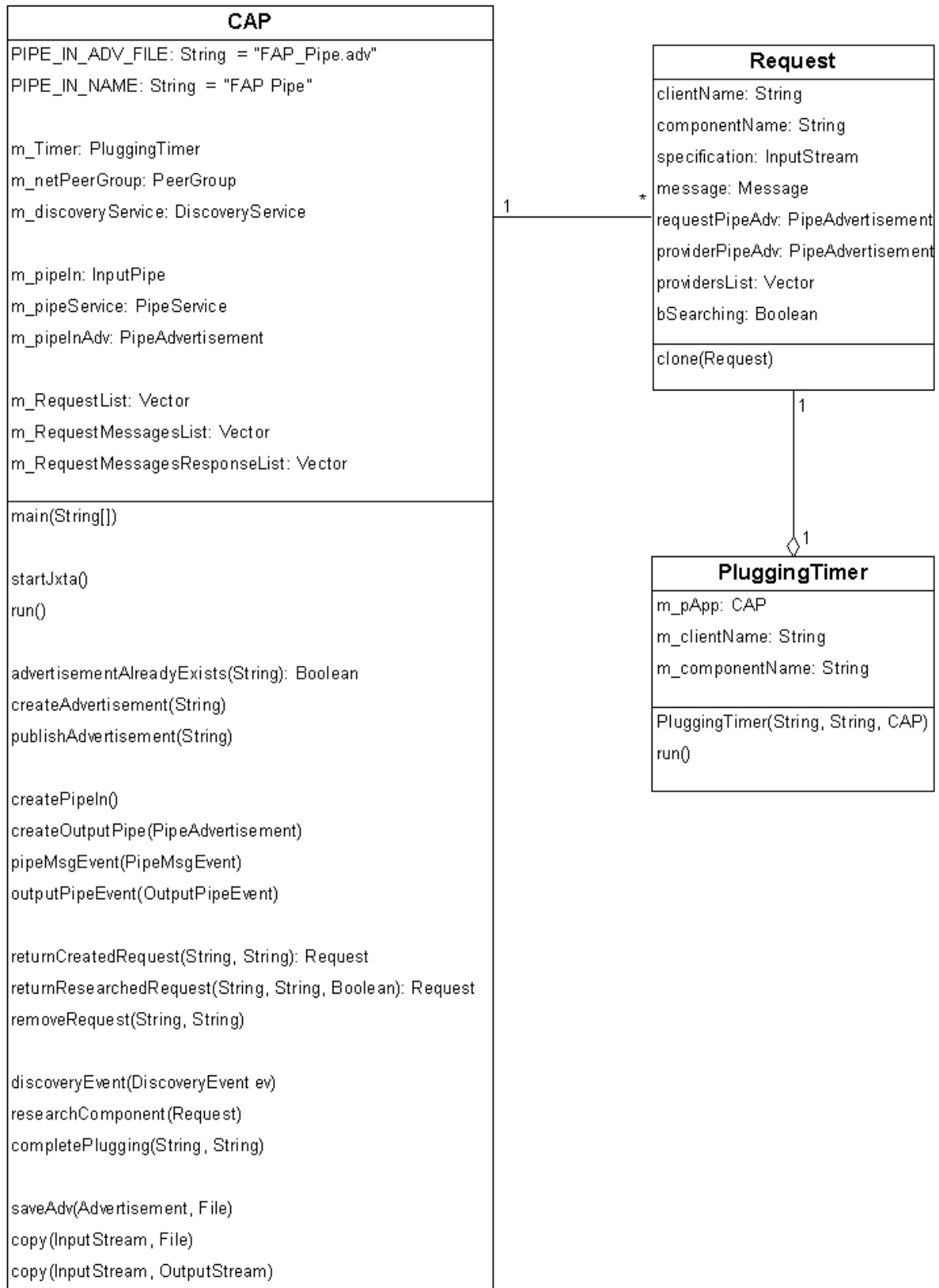
Figura 4.7 – Diagrama de Classes – PAC
