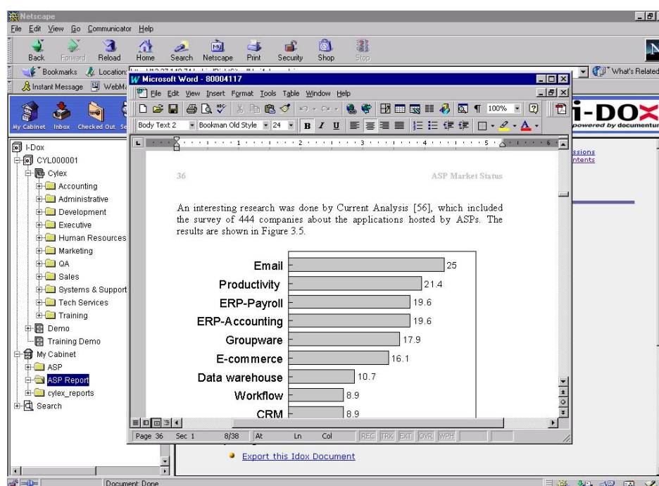
Figura 2.8 – I-DoX (Cylex, 2001)
