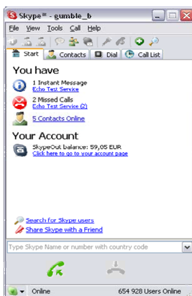
Figura 2.12 – Skype (Skype, 2004)
