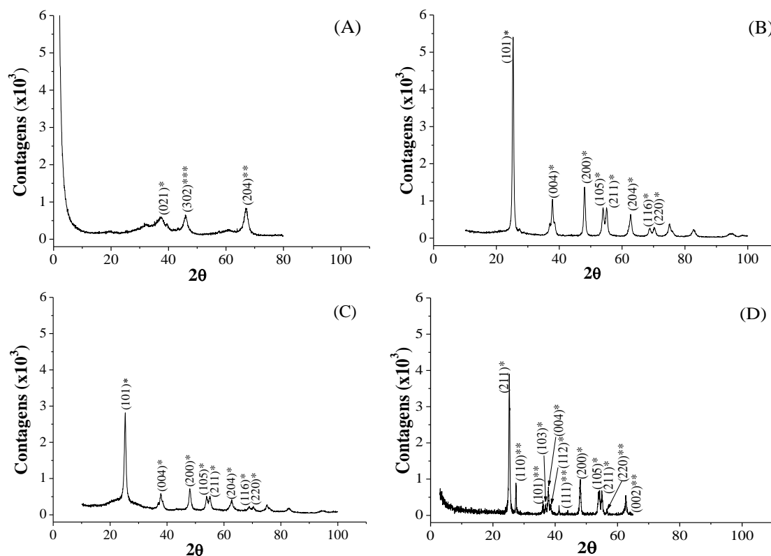
Figura 35. Difratograma de; (A) \text{Al}_R/\text{Ti} ; (B) CCT50%; (C) CCT25%; (D) \text{TiO}_2/\text{P-25} ; (* = anatase, ** = rutilo, *** = broquite; [131, 132]).
