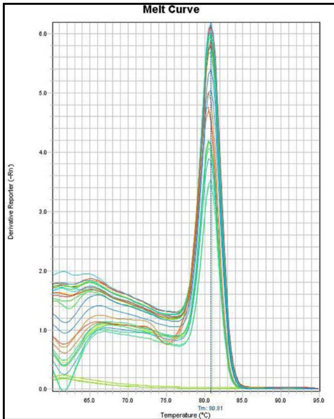
Figure 4. The melt curve of real time PCR reaction, showing the specificity of the reaction.
