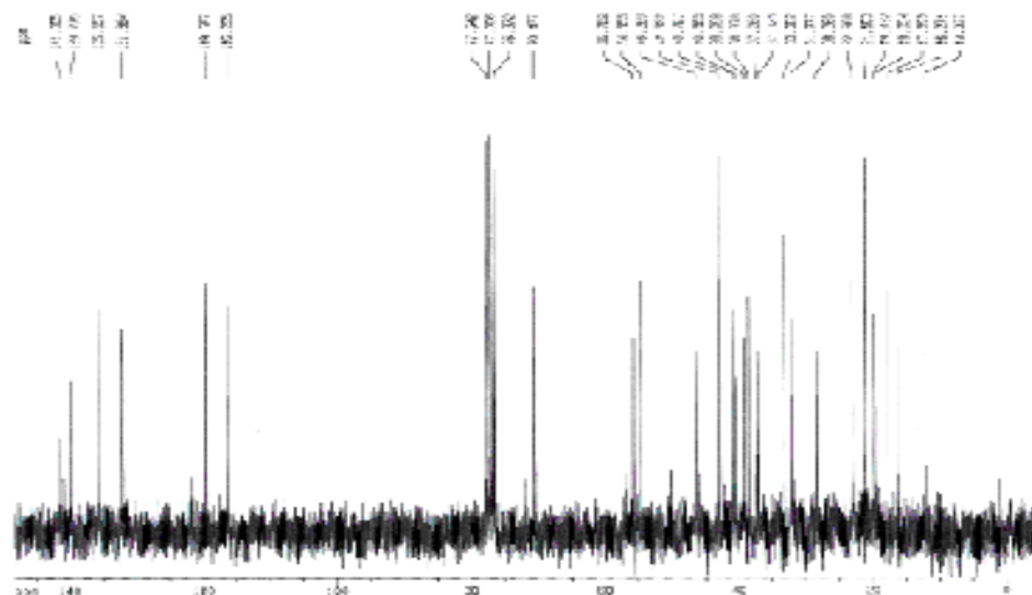
FIGURA 4.70: Espectro de RMN ^{13}\text{C} de S9 (100 MHz, \text{CDCl}_3 )
