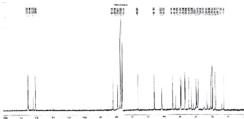
FIGURA 4.71: Espectro de RMN ^{13}\text{C} de S10 (50 MHz, \text{CDCl}_3 )
