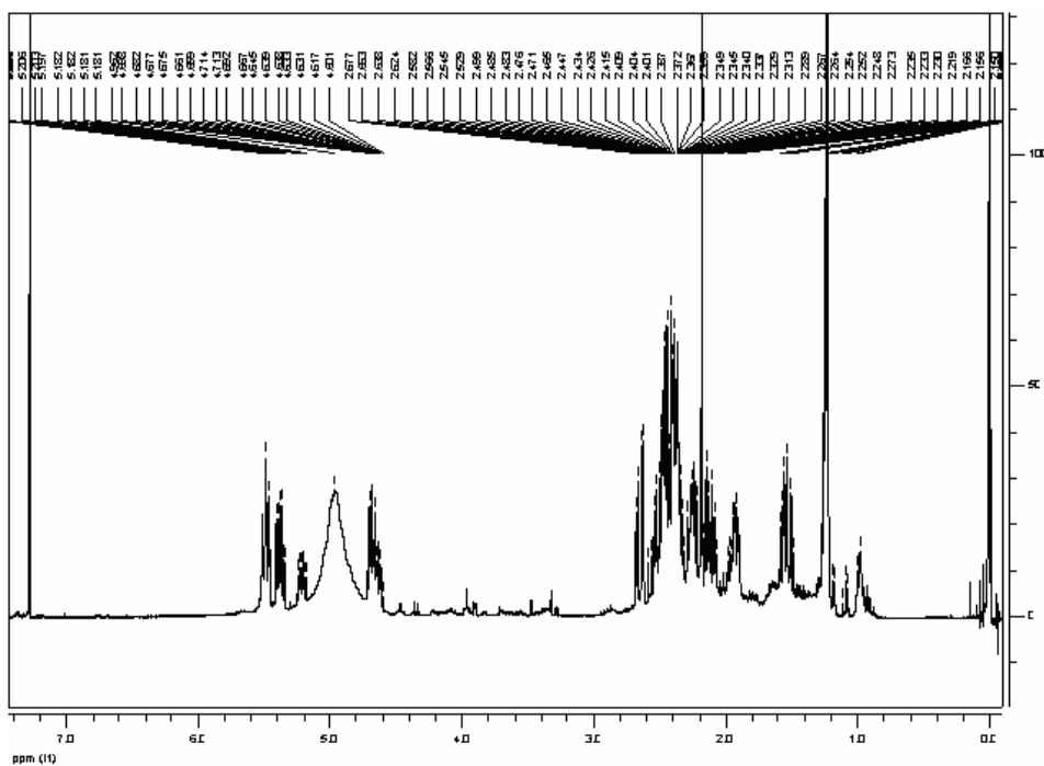
FIGURA 4.51: Espectro de RMN ^1\text{H} de S6 (400 MHz, \text{CDCl}_3 )
