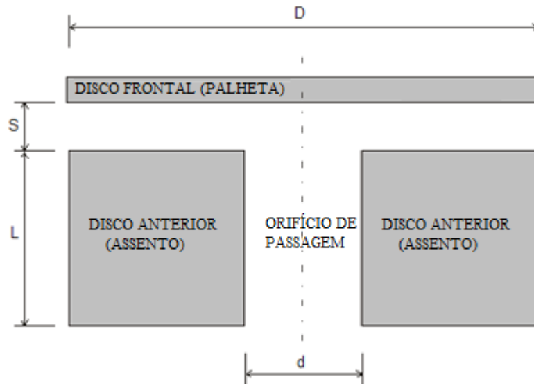
Figura 1.2 – Difusor radial.
