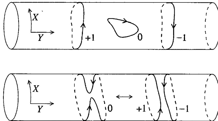
Figure 3.2 Closed oriented strings of winding numbers w=-1, 0, 1 and the transition from a w=0 string to w=-1 and w=+1 strings. In this case, we have one compact dimension X and one non-compact dimension Y . Figure Credits: Joseph Polchinski. String Theory: An Introduction to the Bosonic String (Cambridge Monographs on Mathematical Physics), volume 1. 1998.
