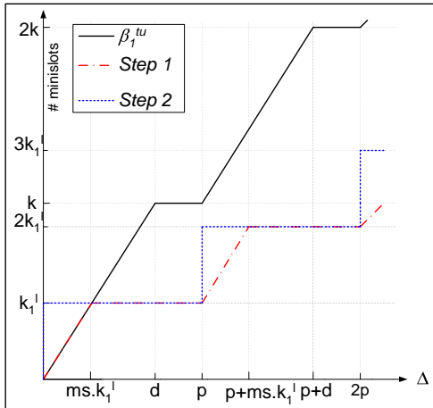
Figura 3.14: Passos 1 e 2 para obter \beta_1^u (CHOKSHI; BHADURI, 2010)
