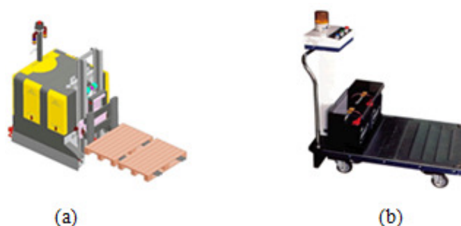
Figura 3.2. Tipos de AGVs: (a) carga de pallet (ELETTRIC80, 2009), (b) cargas leves (AUTOMOTION, 2009)
