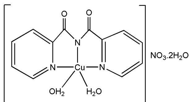
Figura 7 - Estrutura do precursor [\text{Cu}(\text{bpca})(\text{H}_2\text{O})_2]\text{NO}_3 \cdot 2\text{H}_2\text{O} .
