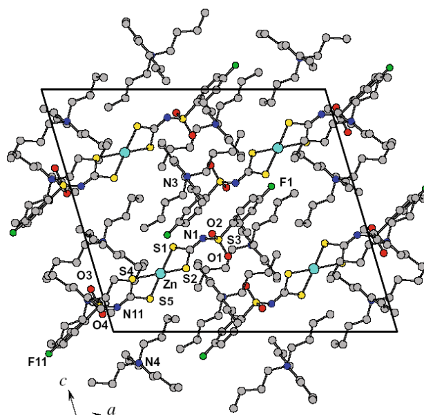
Fig. 4. Molecular arrangements of the compound 2 in the unit cells.
