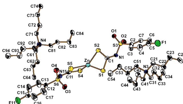
Fig. 3. View of the molecular structure of 2 with labelling of the atoms and the thermal ellipsoids at the 30% probability level. Hydrogen atoms are omitted for clarity.
