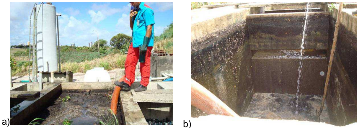
Figura 3.24: Decanto digestor
