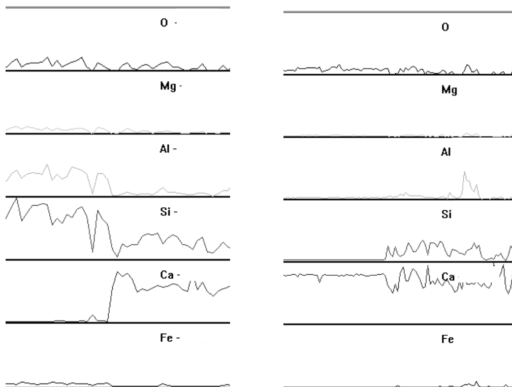
(a) lightweight concrete – 40 MPa (b) normal-weight concrete – 40 MPa Figure 8. 8 - Graphs of the EDS analysis along the lines.
