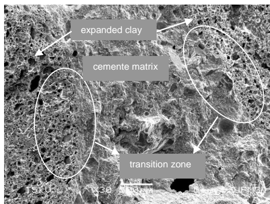
(a) lightweight concrete 40 MPa (30X)
