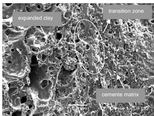
(c) lightweight Concrete - 40 MPa (300X)
