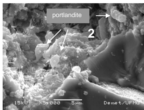
(b) normal-weight concrete – 40 MPa
