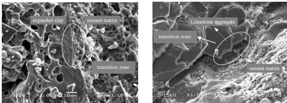
(e) lightweight Concrete - 40 MPa (1000X) (f) normal-weight concrete - 40 MPa (1000X) Figure 8. 4 - Image analysis obtained by scanning electron microscopy.
