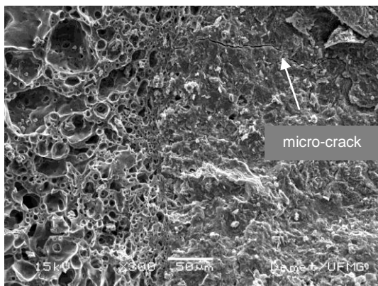
(c) lightweight concrete (300X)
