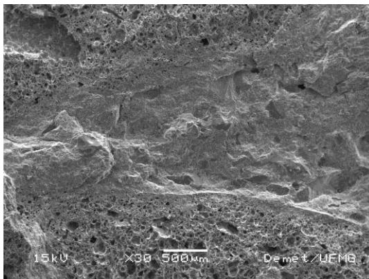
(a) lightweight concrete (30X)
