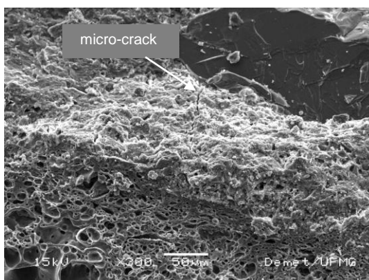
Figure 9. 6 - Transition zone of the aggregates with cement matrix.
