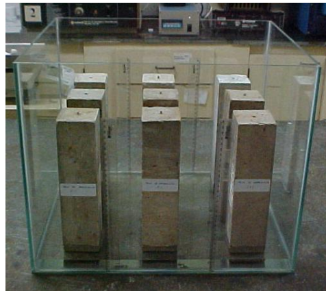
Figure 7.1 - Prismatic specimens in contact with the sheet of water of 10 mm.
