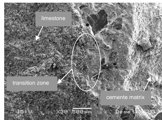
(b) normal-weight concrete 40MPa (30X)
