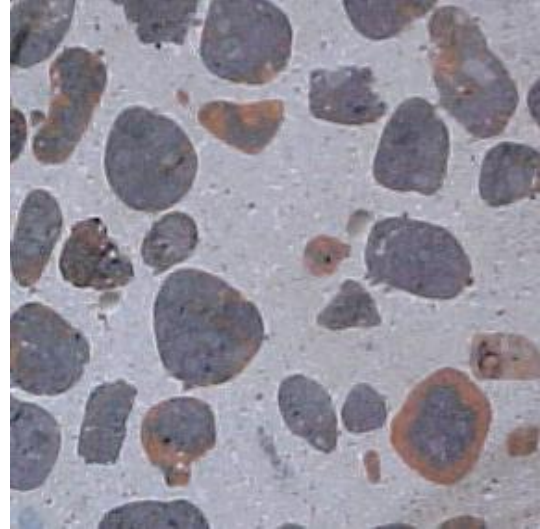
(b) image of the transversal section of LWAC
