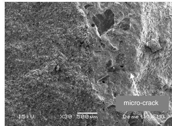
(b) Normal-weight concrete (30X)
