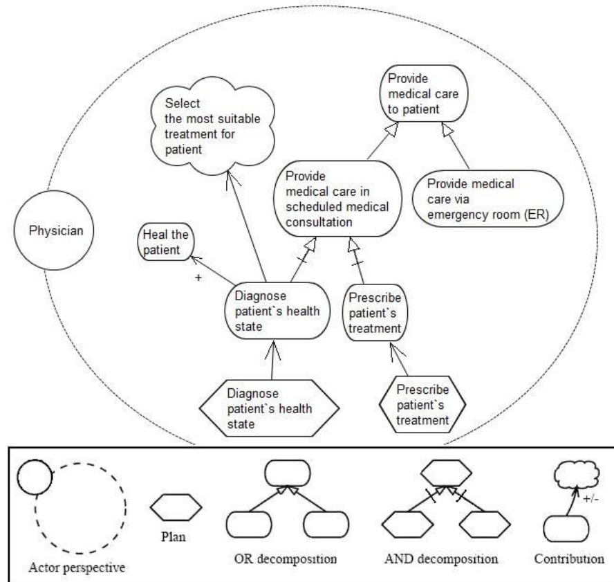
Figure 3.2 Examples of the relationships of the Tropos methodology
