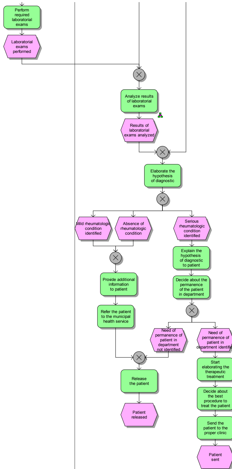
Figure 5.7 The Diagnose patient's health state process model
