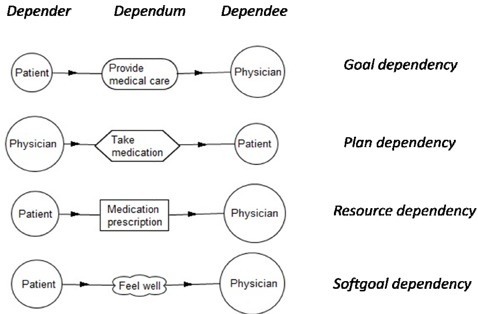
Figure 3.1 Types of dependencies of Tropos methodology
