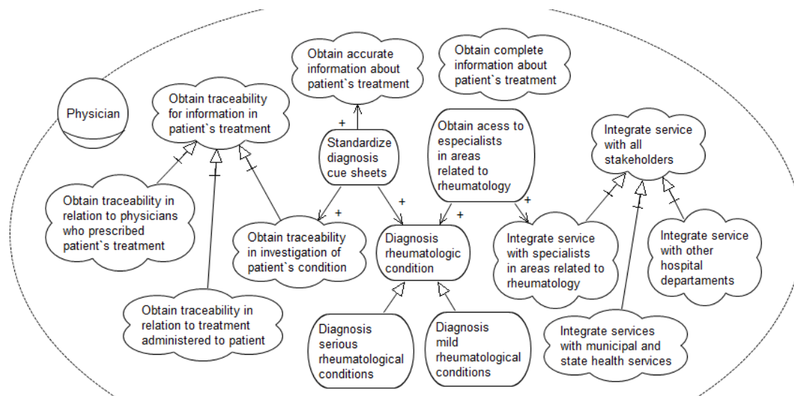
Figure 5.5 Portion of the goal model obtained in goal elicitation activities with catalogues (1)
