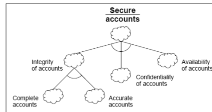
Figure 5.2 Further decomposition of a security softgoal (adapted from (CHUNG et al., 2000) )
