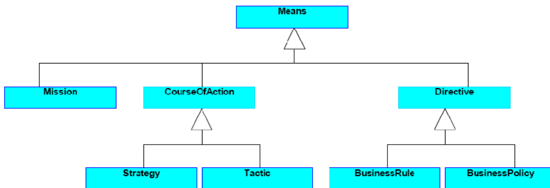
Figure 3.5 The Hierarchy of Means concepts
