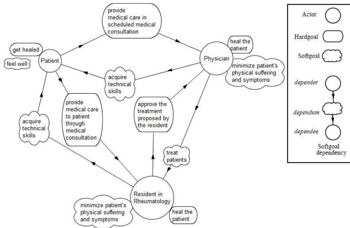
Figure 6.4 An actor diagram in Tropos, depicting a global vision of the organizational scenario
