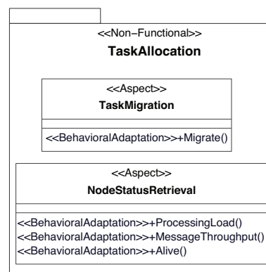
Figure A.5: TaskAllocation Package : dealing with tasks allocation non-functional requirements
