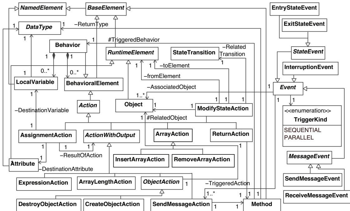
Figure 6.3: DERCS meta-model: behavioral elements
