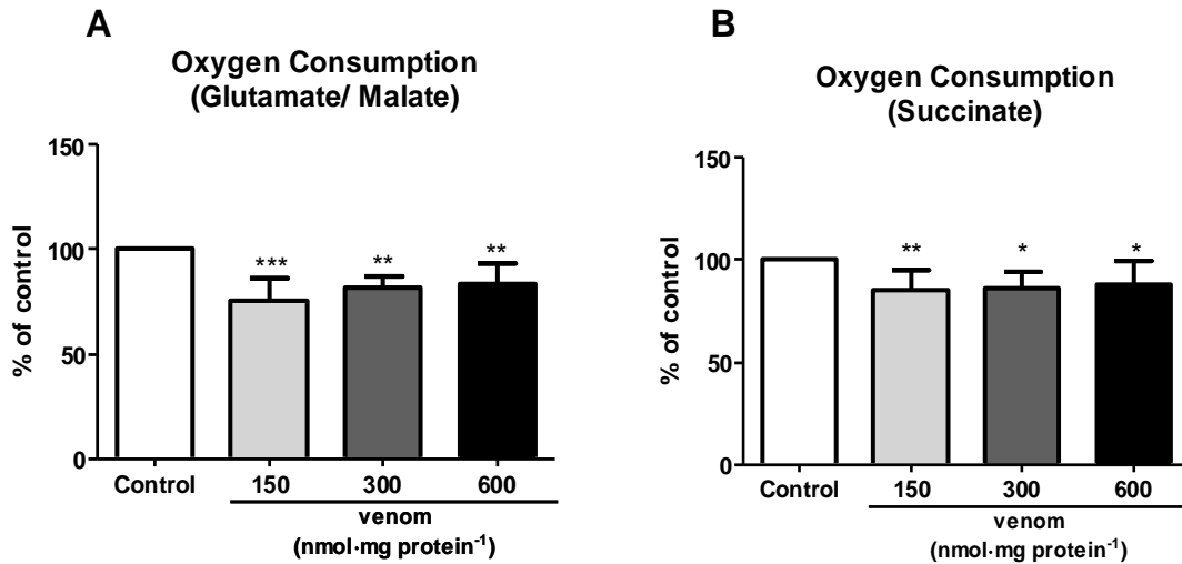
Figure 3. Effect of Cdt venom on oxygen consumption of uncoupled mitochondria. The substrates were glutamate plus malate (A) or succinate (B). Oxygen uptake was determined in isolated liver mitochondria of healthy and untreated rats as described in Material and Methods. Bars show the mean \pm mean standard errors of the percentage of Control. In (A) 100% of activity corresponds to 29.58 \pm 3.26 nmol oxygen consumption per min per mg of protein; in (B) 100% corresponds to 27.66 \pm 4.61 nmol oxygen consumption per min per mg of protein. Symbols: **, statistically different from the control group (* p \leq 0.05 , ** p \leq 0.01 , *** p \leq 0.001 ).
