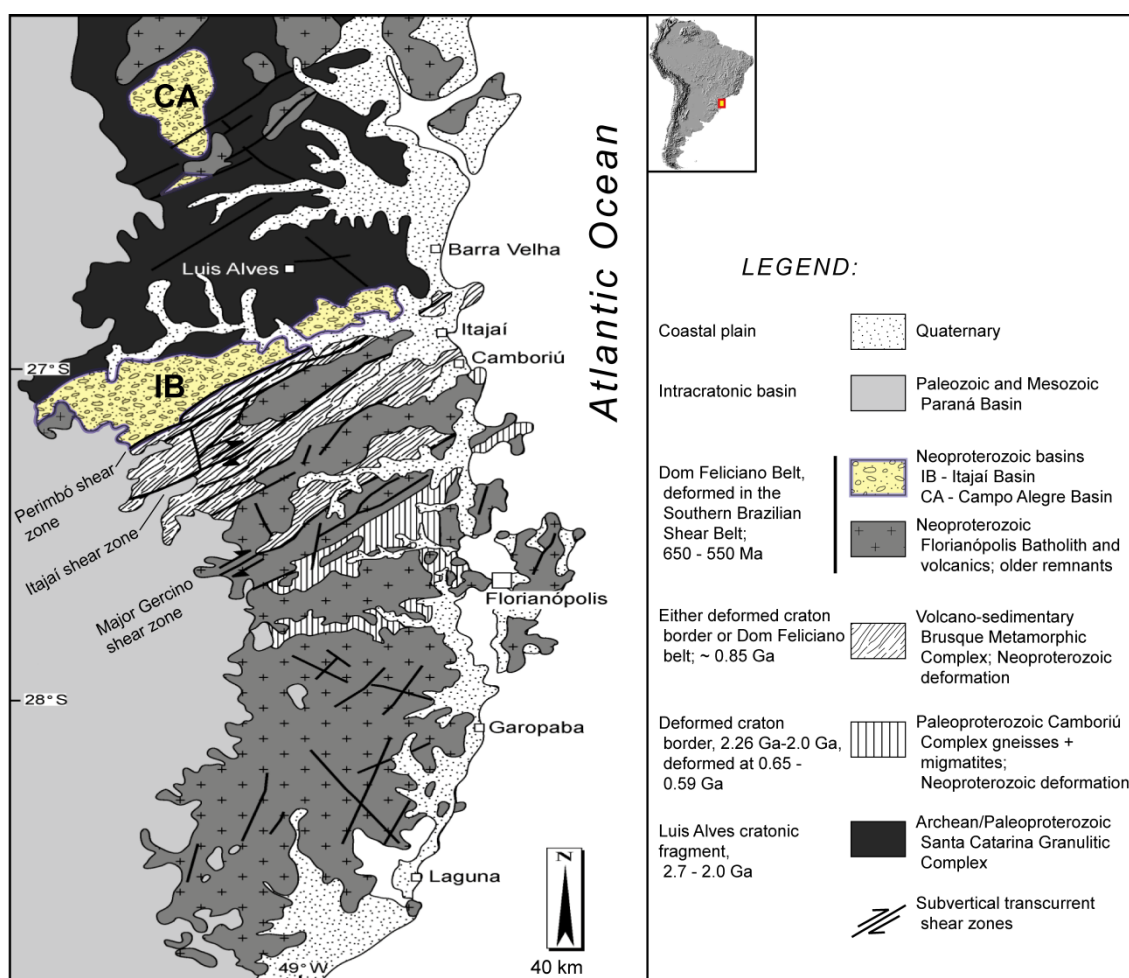
Figure 2: Geological map of the eastern portion of the Santa Catarina State, showing the exposed region of the Catarinense Shield. In yellow are represented the Neoproterozoic basins (Itajaí and Campo Alegre Basins) (modified from Hartmann et al., 2003).
