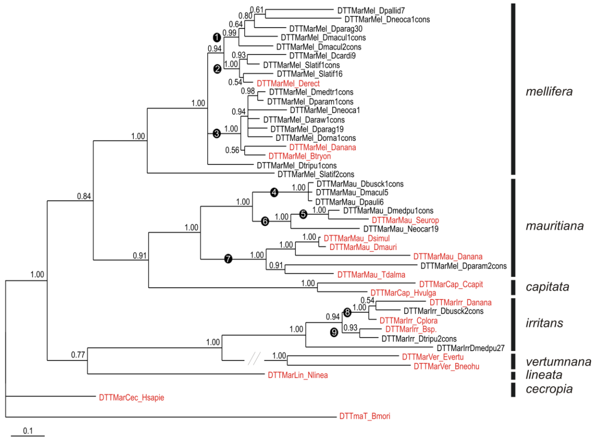
Figure 1: Phylogeny of mariner -like sequences using a Bayesian analysis with the JTT+G model. Posterior probabilities of clades are shown next to the branches. The names in red are sequences obtained in databank (NCBI) and in black are sequences produced in this study. The black bars in right of figure are the subfamilies of mariner Family. The black circles with a white number are the clusters cited in the text.
