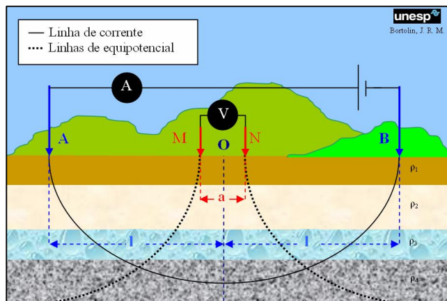
Figura 2.10: Arranjo Schlumberger.
