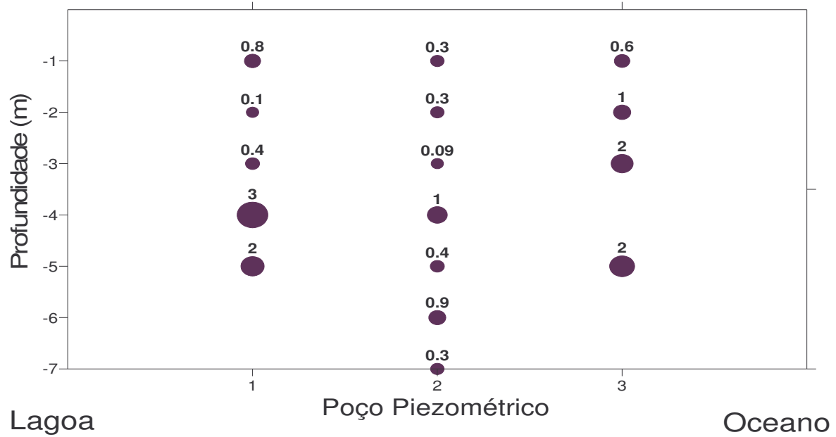
INVERNO - Pb (ppb)
