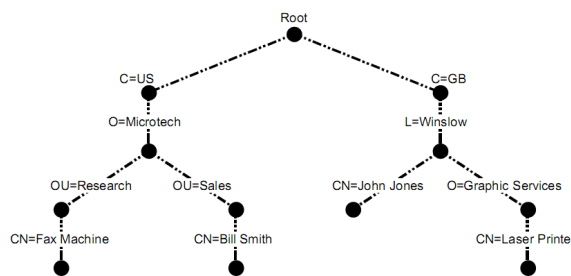
Figura 6: Directory Information Tree .
