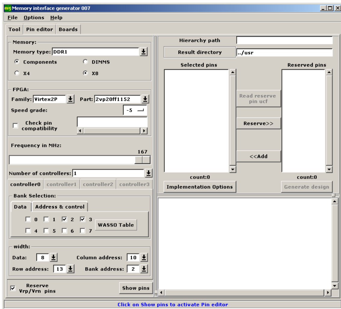
Figura A.1: Interface do Memory Generator Interface .
