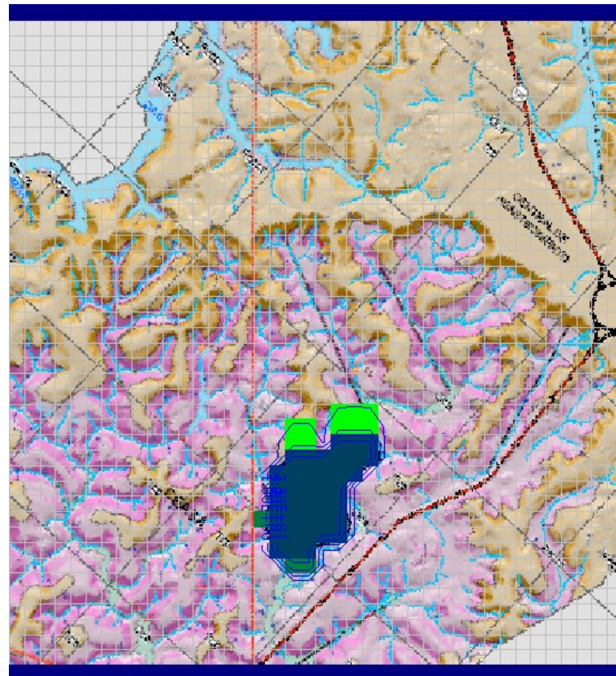
(b) Langmuir
