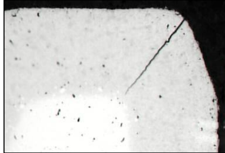
Figure 2: Crack on nitrided stainless steel piston ring, without etch. (500X)
