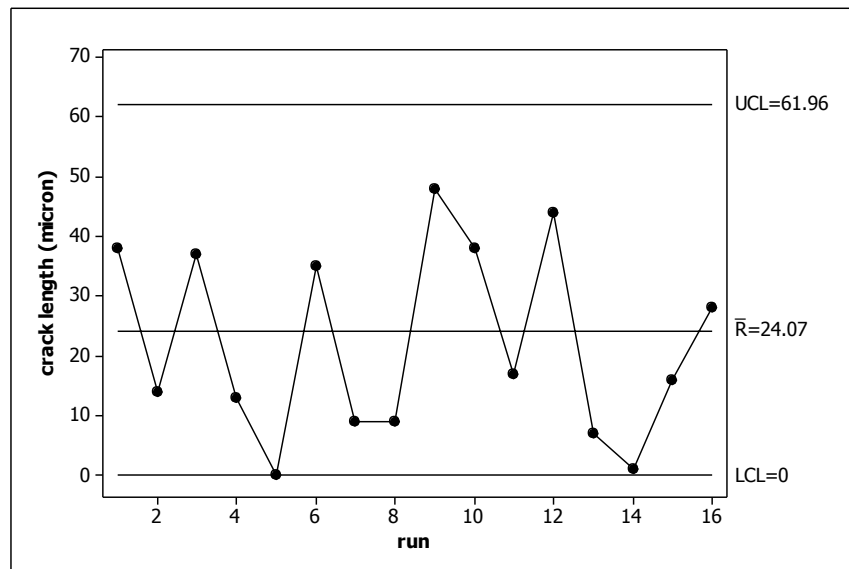
Figure 5: R control chart.
