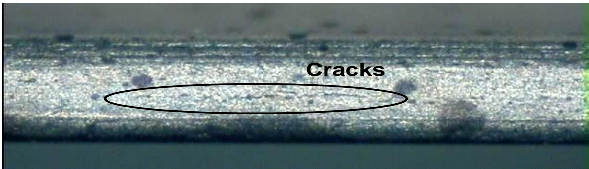
Figure 3: Surface aspect of cracked part. (20X)
