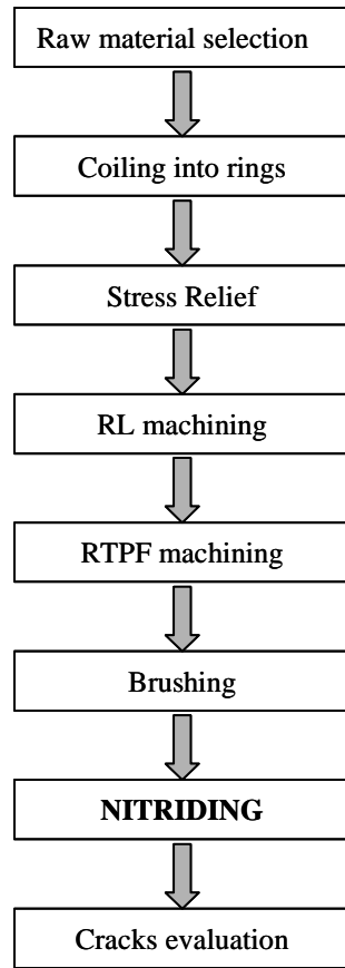
Figure 4 – Process flow.
