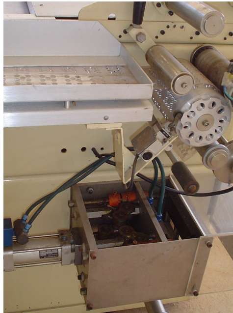
Figura 18: Emblistadeira
