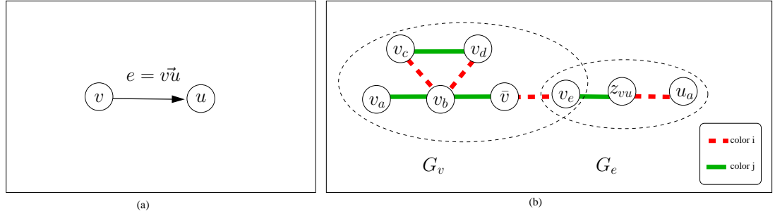
Figure 2.9: (a) Arc \vec{v}u \in V(D) . (b) Gadget G_v associated with vertex v and gadget G_e associated with edge e .
