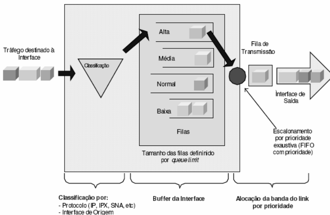
Figura 12: Priority Queueing
