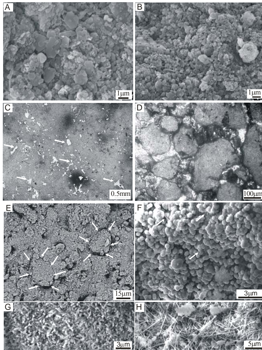
Figure 3.7 Endured mudstones and sandstones representative of the intermediate and semi-flint kaolin units. A,B) Texture of kaolinites from the lower portion of the intermediate kaolin unit, where Kb kaolinites occur in association with Kc kaolinites, with the volume of the latter increasing significantly upward (B) in association with a paleosol horizon.(SEM, secondary electrons). C) Kaolinitized mudstone of the semi flint unit, characterized by a massive texture and displaying fractures and fenestrae filled by clear kaolinite (arrows) (parallel polars). D) Kaolinitized sandstone of the semi flint unit, consisting of sub-rounded to rounded, very fine to medium grains sizes composed by dark brown Kc kaolinites coated by iron oxides. Note the clear kaolinite cementing the interstitial space (bright color) (parallel polars). E) Sandstone from the semi-flint unit, characterized by a strongly kaolinitized fabric, but where sand grains can be distinguished (arrows) from the “matrix” of similar composition (SEM, back scatter). F) A detail of the interstitial space of a sandstone from the semi-flint unit, cemented by spherules of iron oxides. Note a few hairy crystals of halloysite (arrows) (SEM, secondary electrons). G, H) Details of tabular (G) and hairy (H) halloysite crystals that occur cementing the kaolinitized sandstones of the semi-flint unit (SEM, secondary electrons).
