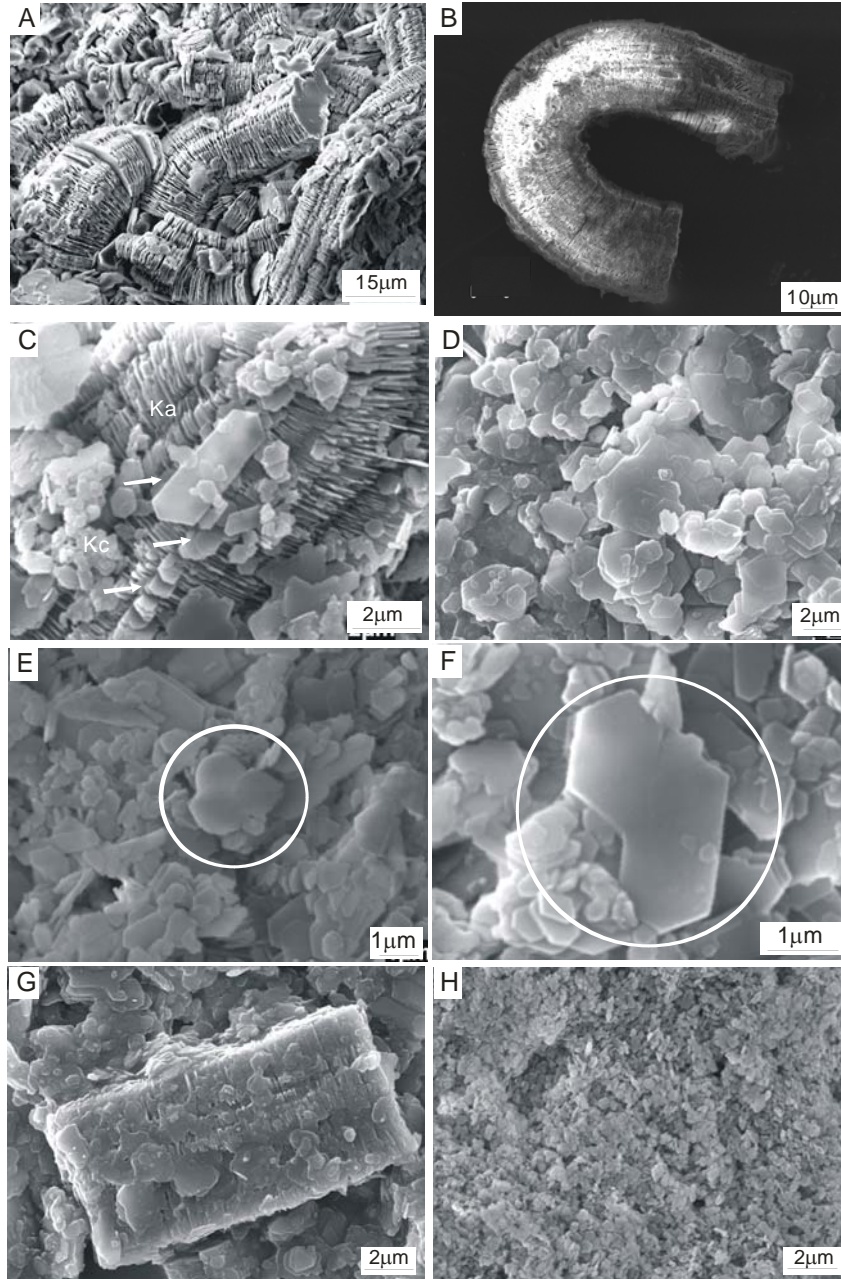
Figure 3.6 Kaolinite from the soft kaolin unit. A) Agglomerate of Ka kaolinites, consisting of booklets of hexagonal to pseudo-hexagonal crystals up to 30 \mu\text{m} in diameter. B) U-shaped, vermicular Ka kaolinite. C) A booklet of Ka kaolinite with superimposed prismatic rectangular crystals that grow out from the kaolinite sheets. Note the local agglomerate of Kc kaolinite in the lower left side of the picture. D) Kb kaolinite composed by hexagonal and pseudo-hexagonal crystals averaging 1-3 \mu\text{m} in diameter. E) Kb kaolinite, consisting of crystals with face-to face arrangement (circle). F) Kb kaolinite, consisting of crystals with parallel to pseudo-parallel arrangement (circle). G) A crudely developed booklet of kaolinite, attributed to result from replacement of a feldspar grain. H) Kc kaolinite, consisting of hexagonal to pseudo-hexagonal crystals with regular size around 200 nm in diameter, typical of the paleosol horizon from the top of the soft kaolin unit.
