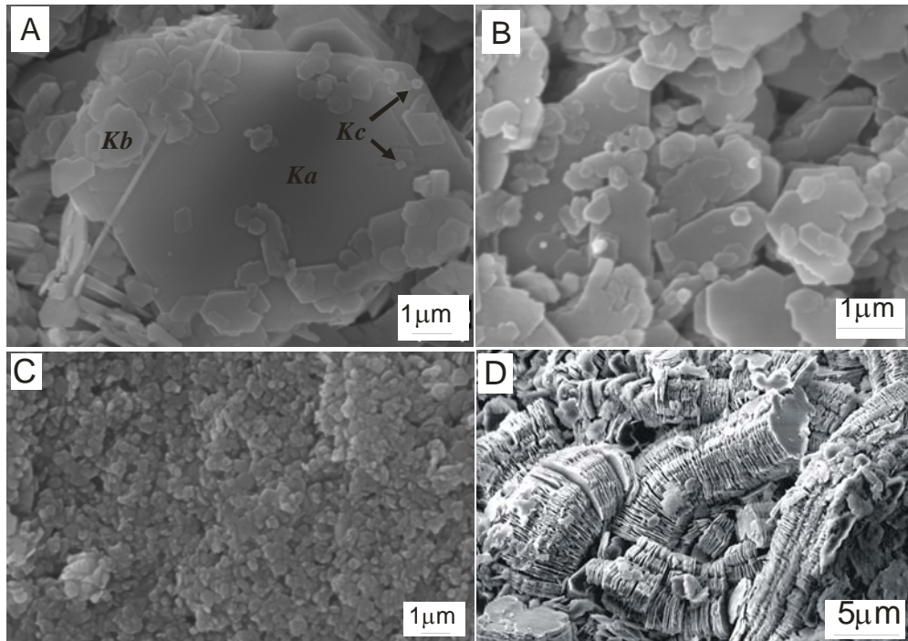
Figure 4.2 Types of kaolinites from the Rio Capim area. A-B) Ka and Kb kaolinites, typical of sandstones (A) and mudstones (B) of the soft kaolin unit, respectively. C) Kc kaolinite, typical of the semi-flint kaolin unit. D) Kaolinite booklets.
