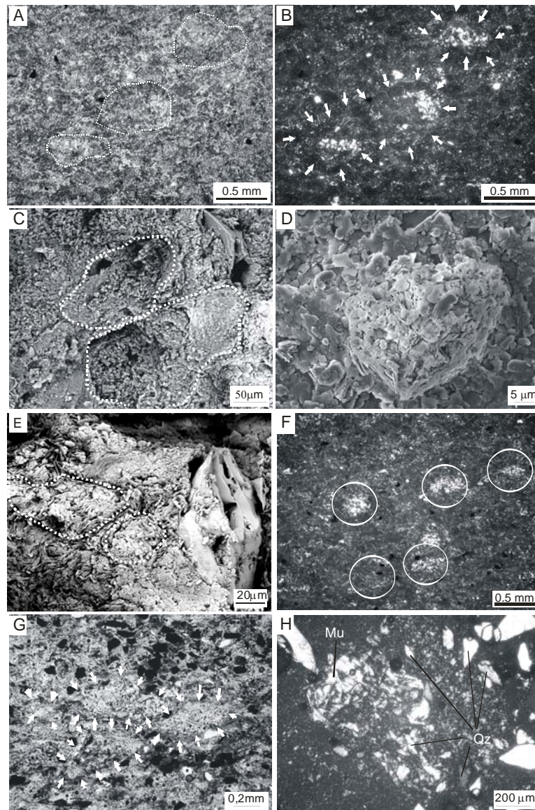
Figure 3.4 Kaolinitized sandstone, representative of the middle and upper portion of the soft kaolin unit. A-B) A view of an intensely kaolinitized framework with parallel (A) and crossed polars (B), where the contours of well rounded grains are still preserved (hatched lines and arrows in A and B, respectively). Note many relics of a mineral (cristobalite?; light color) not replaced by kaolinite. C) SEM view (back scatter) of the framework, highlighting two, well rounded, kaolinitized sand grains (hatched lines). D) A detail of a grain completely replaced by Kb kaolinites crystals (SEM, back scatter). E) Bipyramidal quartz within a kaolinitized framework with two ghosts of sand grains (SEM, back scatter). F) Bipyramidal-shaped cristobalite (?; circles) floating within a kaolinitized “matrix”, which might represent either individual euhedral grains or crystals from lithic grains that were left behind during kaolinitization (crossed polars). G) Kaolinitized bipyramidal grains (arrows), with numerous black inclusions, probably a product of replacement of the grains by kaolinite (crossed polars). H) A detail of a large, kaolinitized lithic grain with relics of pyramidal quartz and muscovite crystals (crossed polars).
