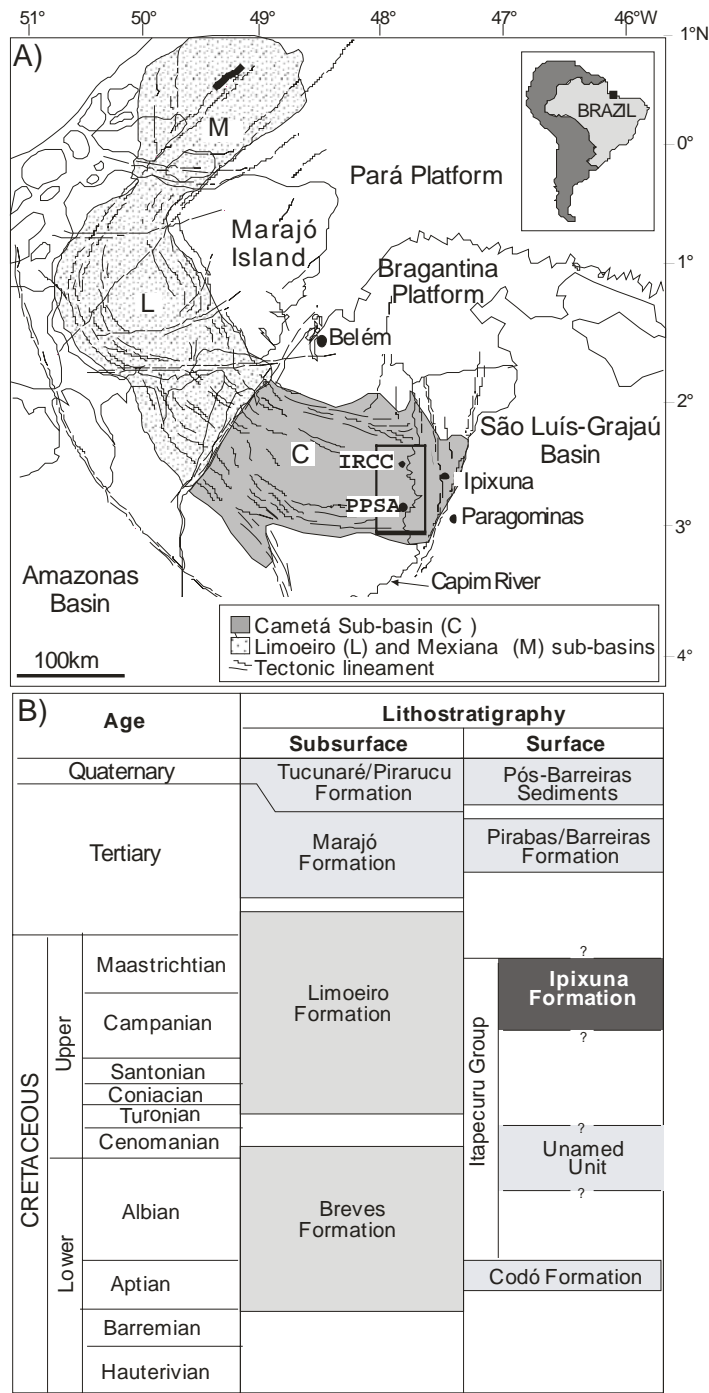
Figure 2.1: A) Location map of the study area in the Rio Capim area, Cameté Sub-Basin, with the studied kaolin quarries PPSA and RCC indicated. B) Stratigraphic chart representing the sedimentary successions in the Cameté Sub-Basin, both in the subsurface and surface exposures.
