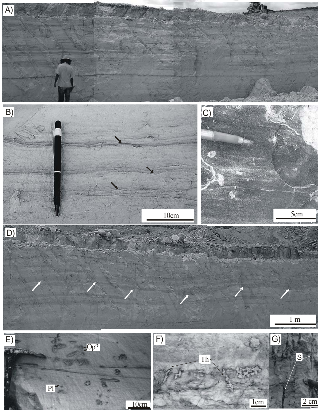
Figure 2.6: Upper flow regime tidal sand flat/sand bar (Facies Association D). A) General view of an outcrop illustrating tabular sandstones with horizontal to low-angle dipping cross stratification (Facies St) (man=1.65 m tall). B) Horizontal lamination with laminae highlighted by heavy minerals. C) Sandstone with parting lineation (pencil oriented parallel to paleoflow). D) Undulating lamination forming scour or swales locally filled by mudstone (white arrows). E-G) Trace fossils, representative of the upper flow regime tidal sand flat/sand bar. Thalassinoides (Th), Planolites (Pl) and Skolithos (S) and Ophiomorpha (Op).
