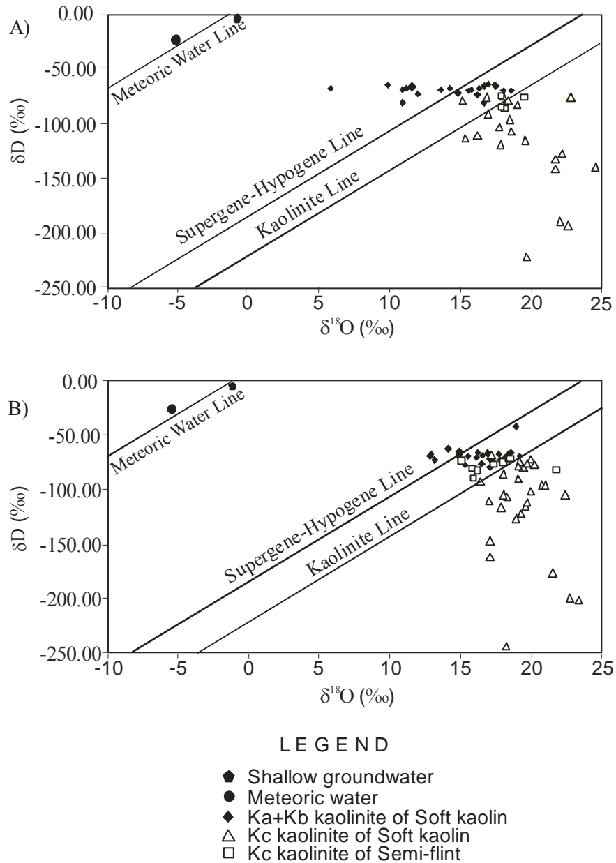
Figure 4.5 Binary diagram with plots of \delta D and \delta^{18}O isotopic values of the kaolinites of the study area, as well as of the modern meteoric water and groundwater. Also plotted are the kaolinite line (Savin and Epstein, 1970a), the supergene/hypogene line (Sheppard et al. , 1969) and the meteoric water line (Craig, 1961). See text for discussions.
