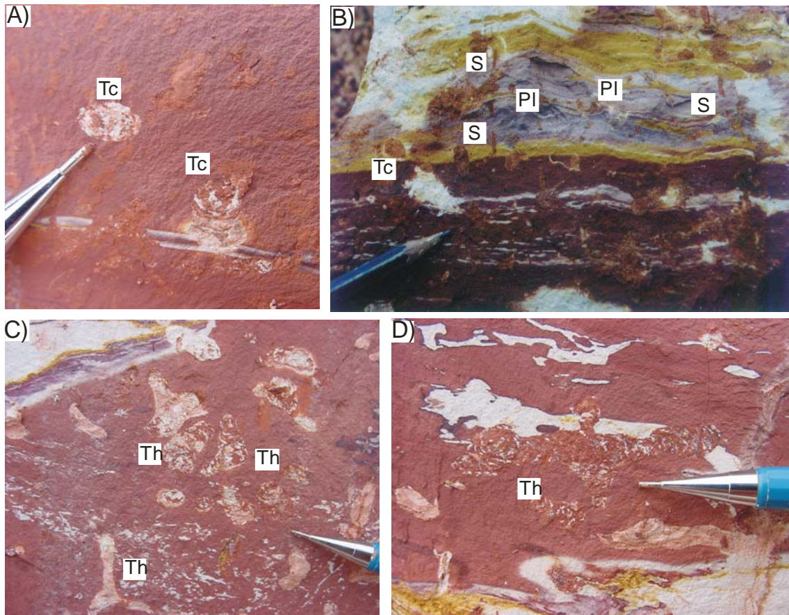
Figure 2.5: A-D) Details of trace fossils representative of tidal channel (Facies Association B) and tidal flat/mangrove deposits (Facies Association C): Thalassinoides (Th), Planolites (Pl), Teichichnus (Tc) and Skolithos (S).
