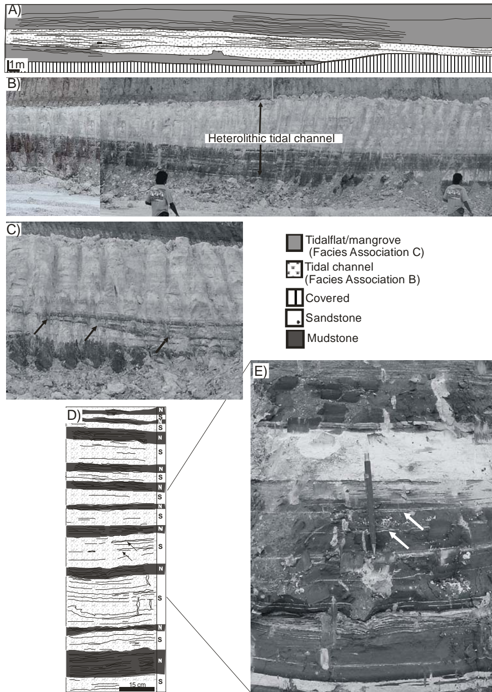
Figure 2.4: Tidal channel (Facies Association B) and tidal flat/mangrove (Facies Association C). A) Geologic section illustrating the spatial relationship between facies associations B and C. Note the gentle concave upward surface that defines the base of a tidal channel deposit. B) General view of a heterolithic tidal channel deposit (man = 1.65 m tall). Dark color = muddier deposits. C) Detail of the sharp, erosional base of a heterolithic tidal channel. D) Heterolithic deposits typical of facies associations B and C, illustrating a vertical succession attributed to tidal bundles. These consist of rhythmically alternating sandier (spring) and muddier (neap) cycles (S=spring; N=neap). Mud couplets attributed to ebb/flood fluctuation are locally present in some spring cycles (black arrows), and undetermined trace fossils are common (white arrows).
