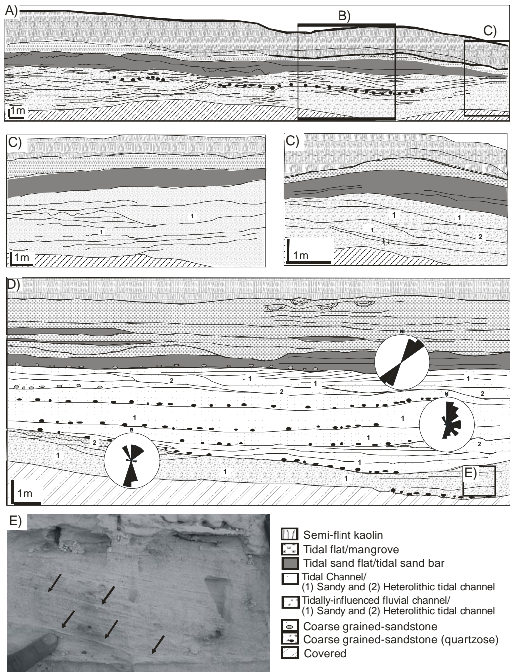
Figure 2.3: A-D) Representative geologic sections, illustrating the sedimentologic characteristics and spatial distributions of facies and facies associations of the soft kaolin unit of the Ipixuna Formation in the RCC quarry. Note that B and C are close-ups of Figure A, illustrating the tidally-influenced fluvial channel deposits (Facies Association A). Observe, also, that D contains rose diagrams with paleocurrent data obtained from cross-stratified sandstones of tidally influenced fluvial channel (Facies Association A) and tidal channel (Facies Association B), as well as parting lineation of upper flow regime tidal sand flat/sand bar (Facies Association D) deposits. E) Close-up photograph of tidal-influenced fluvial channel deposits (Facies Association A), showing foreset packages with mud drapes (arrows).
