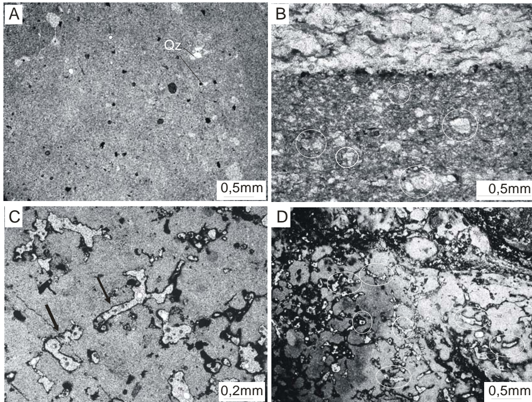
Figure 3.5 Deposits from the top of the soft kaolin unit. A) A general view of massive, kaolinitized mudstone with a few, disperse grains of quartz. B) Heterolithic deposits formed by alternating laminae of light brown to greenish brown siltstone (dark color) and very-fine grained sandstone (light color). Note the relicts of prismatic and/or bipyramidal quartz grains (circles) within the siltstone. C) Kaolinitized mudstone from a paleosol horizon at the top of the soft kaolin unit. Note the several areas cemented by clear kaolinite, related to fractures and/or roots (arrows). D) A reworked deposit from the top of the paleosol horizon, forming sandstone cemented by clear kaolinite (arrows) and iron oxides (black color).
