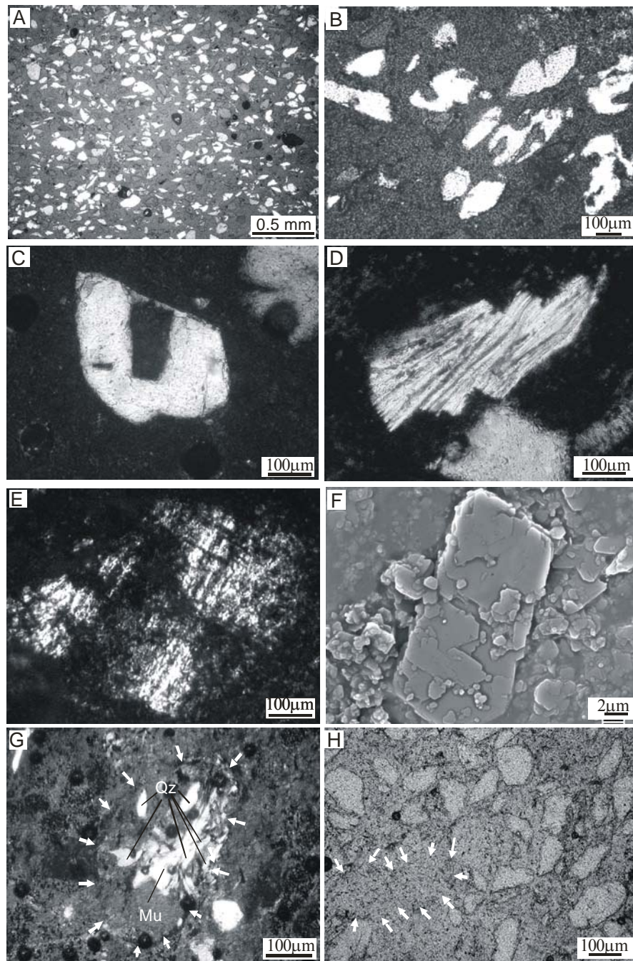
Figure 3.3 Kaolinitized quartzose sandstone, representative of the lower portion of the soft kaolin unit, illustrating: A) a broad view of the framework dominated by monocrystalline quartz grains; B,C) quartz grains with bipyramidal or cuneiform shapes, as well as vacuoles and embayments filled by kaolinite; D) muscovite grain partly replaced by kaolinite; E,F) feldspar grain partly replaced by kaolinite (note the albite twinning and prismatic shape); G) a lithic fragment (arrows) composed by muscovite, cuneiform quartz and a kaolinite, the latter resulting from replacement of other mineralogical constituents of the grain (note that the quartz crystals-Qz are broadly aligned parallel to the maximum elongation axis of the muscovite-Mu); H) ghosts of totally kaolinitized grains (arrows) with texture similar to the matrix. (A-E and G=crossed polars; F=SEM, secondary electrons; H=parallel polars).
