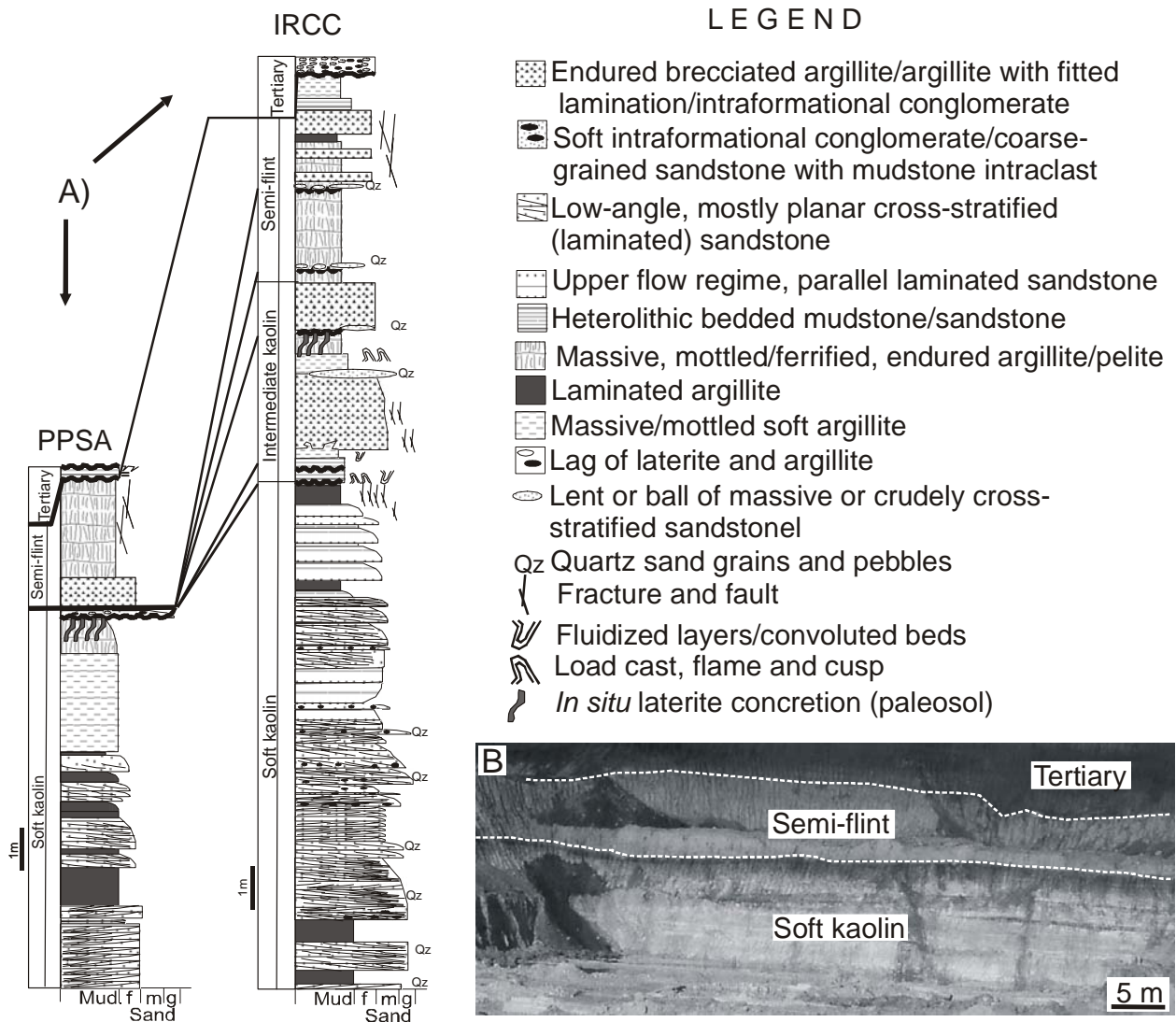
Figure 3.2. A) Lithostratigraphic profiles representative of the Ipixuna Formation in the studied quarries. B) General view of the Ipixuna Formation in the PPSA quarry, illustrating the soft kaolin and the semi flint kaolin units separated by a sharp discontinuity surface, attributed to an unconformity. Note also the unconformity at the top of the semi flint kaolin, which is overlain by Tertiary deposits.
