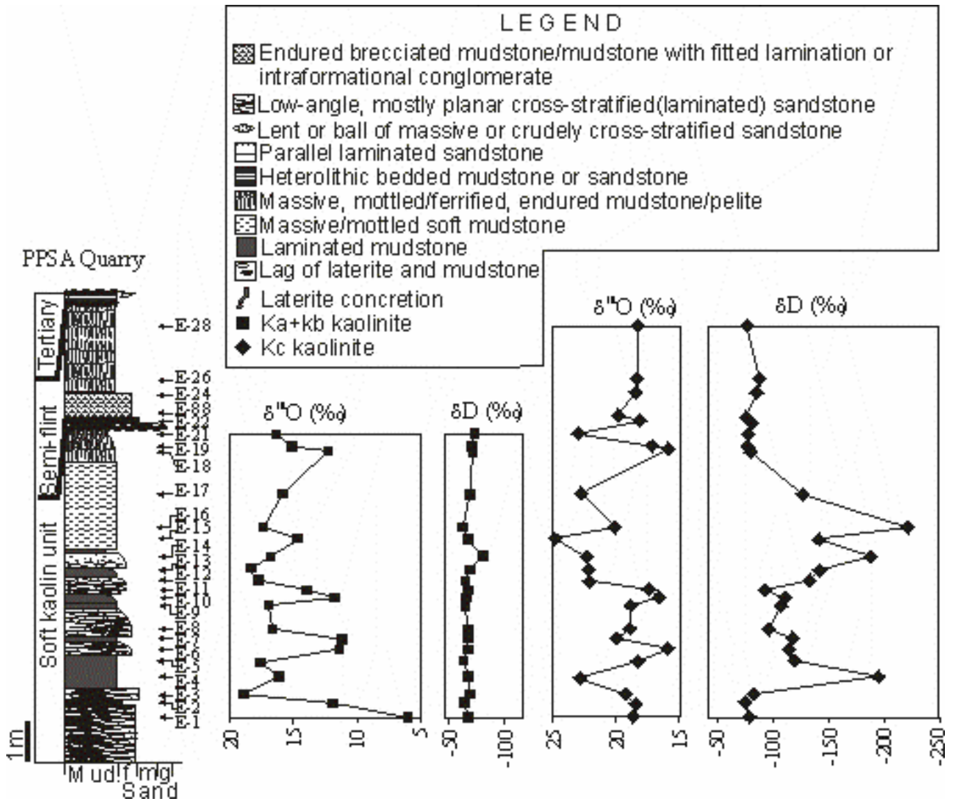
Figure 4.3 Lithostratigraphic profiles of the PPSA quarry, with the corresponding \delta D and \delta^{18}O isotope values.
