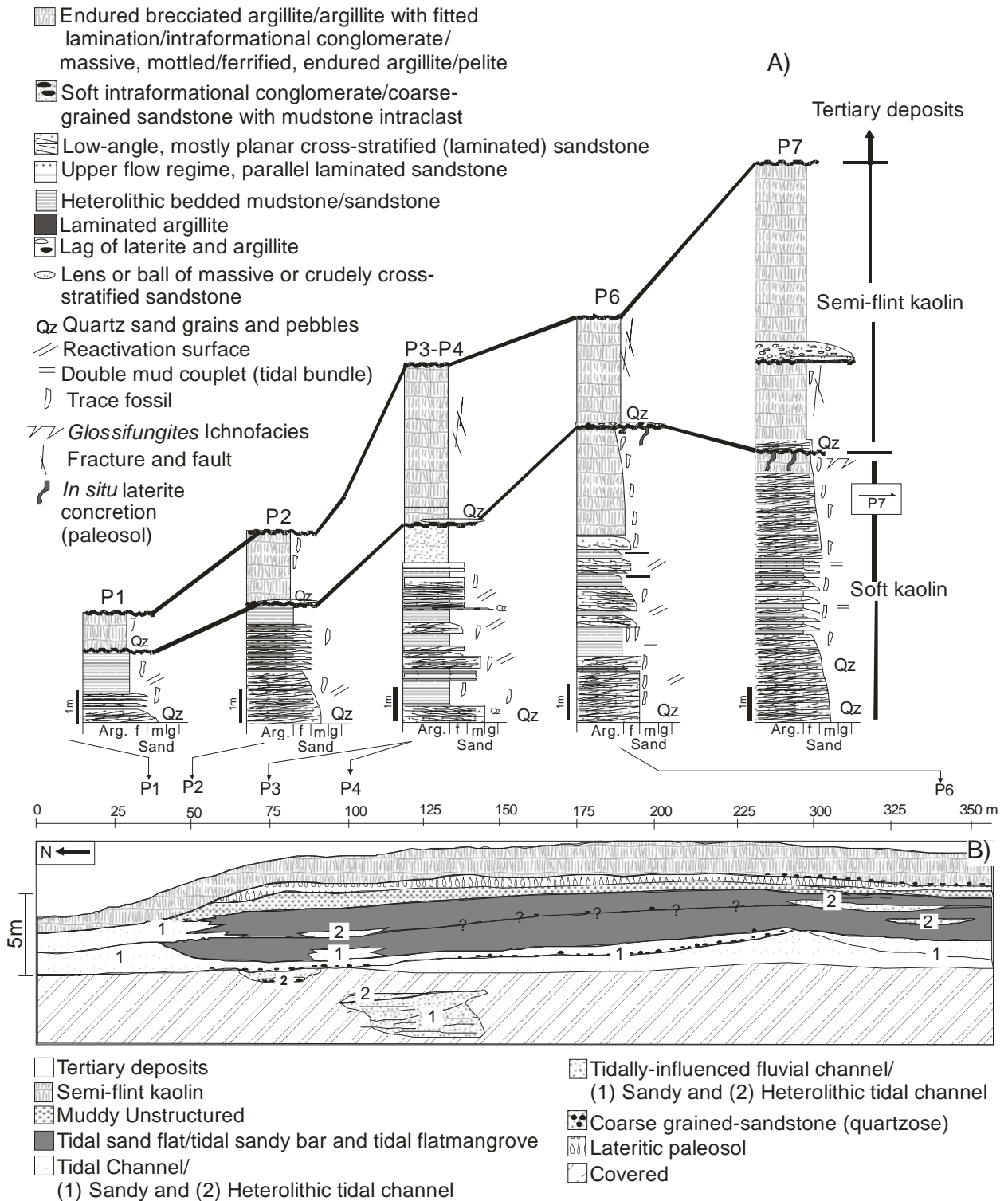
Figure 2.2: Measured lithostratigraphic profiles (A) and geologic cross-section (B) illustrating the sedimentologic characteristics and spatial distributions of facies and facies associations present in the soft kaolin unit of the Ipixuna Formation in the PPSA quarry. Profile P7 is not shown in this geological section, being located circa 200 m to the south.
