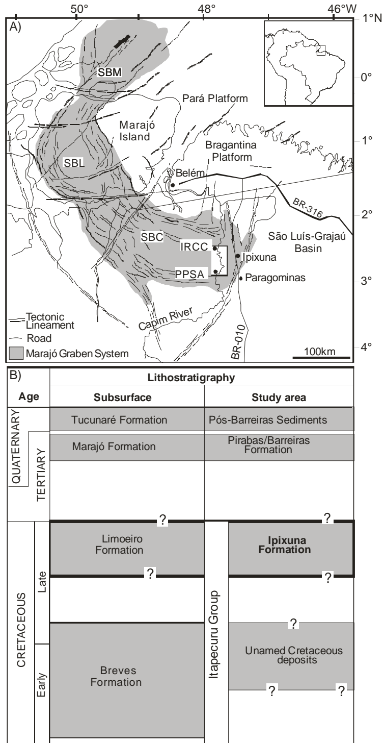
Figure 4.1 A) Location of the study area in the eastern Cameté Sub-Basin, Marajó Graben System, with indication of the two studied quarries, the IRCC and PPSA (SBC=Cameté Sub-Basin, SBL=Limoeiro Sub-Basin, SBM=Mexiana Sub-Basin). B) Lithostratigraphic chart of the Cameté Sub-Basin.
