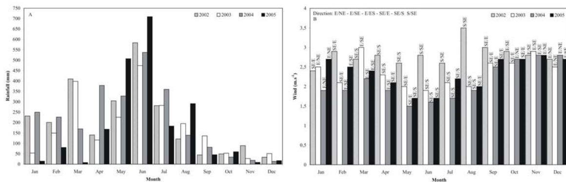
Figure 2. Monthly averages for the Recife station (center): A – rainfall precipitation (mm). B – Velocity (m.s -1 ) and direction of winds.
