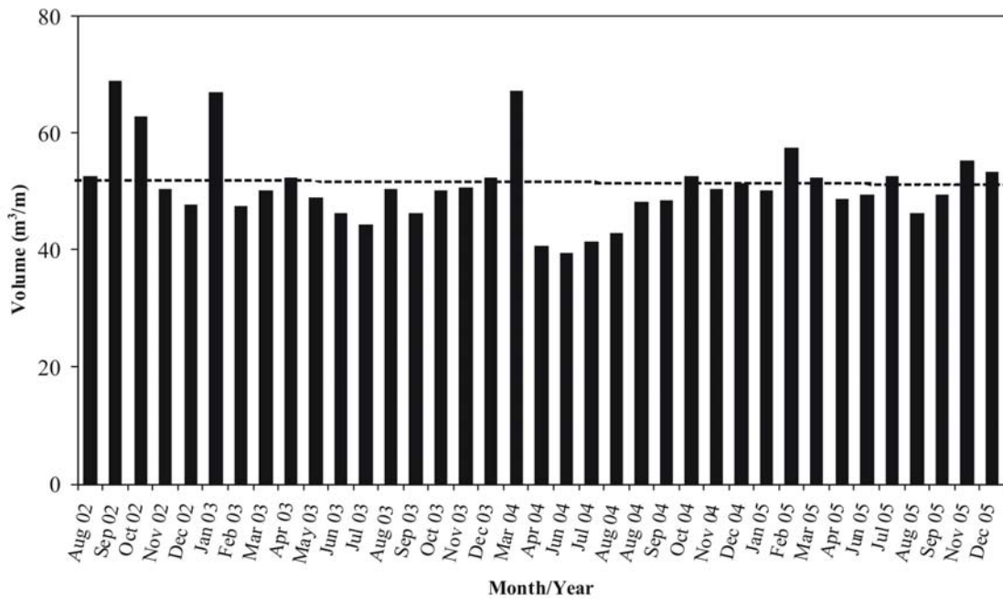
Figure 9. Volumetric variations in profile 5.
