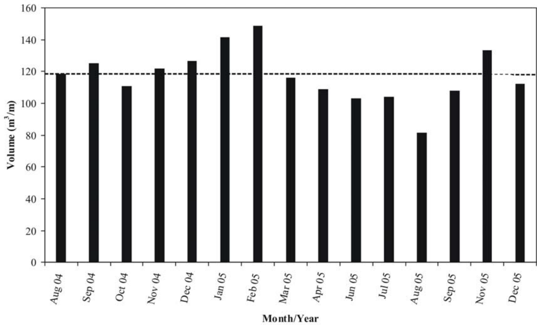
Figure 8. Volumetric variations in profile 4B.
