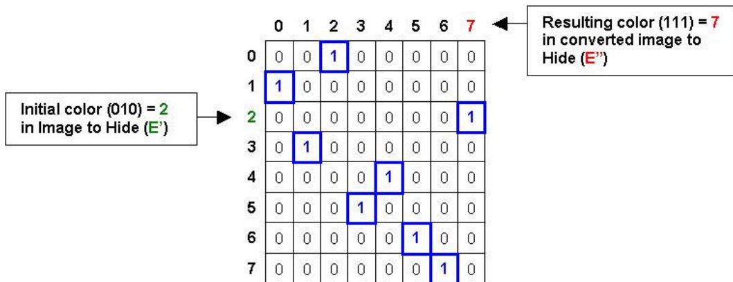
Figure 11 – A three bits substitution matrix sample (k=3)
