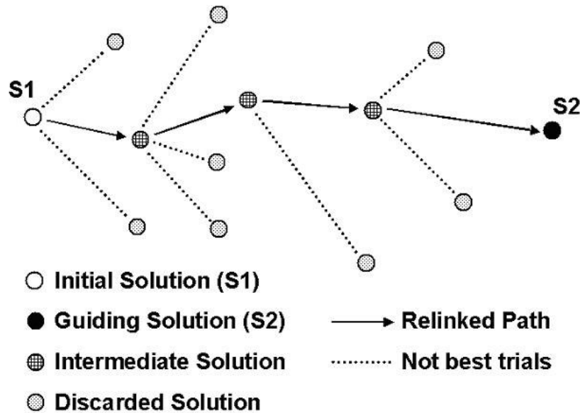
Figure 17 – The path relinking process
