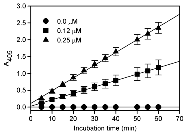
Fig. 3. rPTPηCD specific activity. The purified recombinant rPTPηCD was assayed in triplicates for phosphatase activity toward a substrate, pNPP, at two enzyme concentrations (0.12 and 0.25 μM) and different incubation times (5–60 min). The activity (free phosphate release) is expressed as A 405 . Samples containing no enzyme were used as negative control (filled circles).
