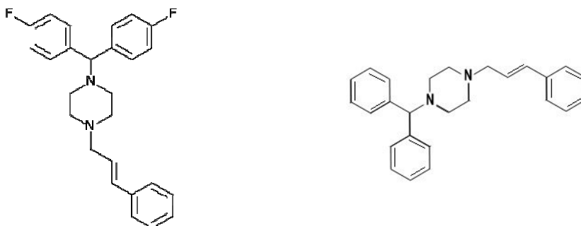
a) Flunarizina ( C_{26}H_{26}F_2N_2 ), MM: 404,5 \text{ g/mol}^{-1} b) Cinarizina ( C_{26}H_{28}N_2 ), MM: 368,5 \text{ g/mol}^{-1}
