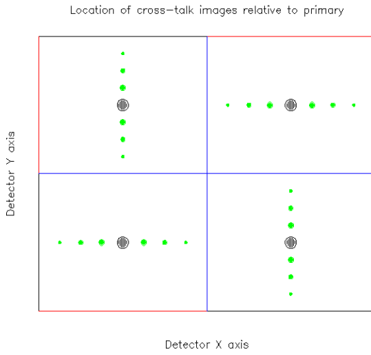
Figure 4.3: Left panel: Diagram showing how the crosstalks appear in different quadrants. The crosstalk pattern rotates because the readout amplifier for each quadrant is located on a different edge of the detector, as shown by the red lines. Right panel: An example of crosstalk detected in one of our images. Whenever there is a saturated star, a crosstalk pattern will be present.
