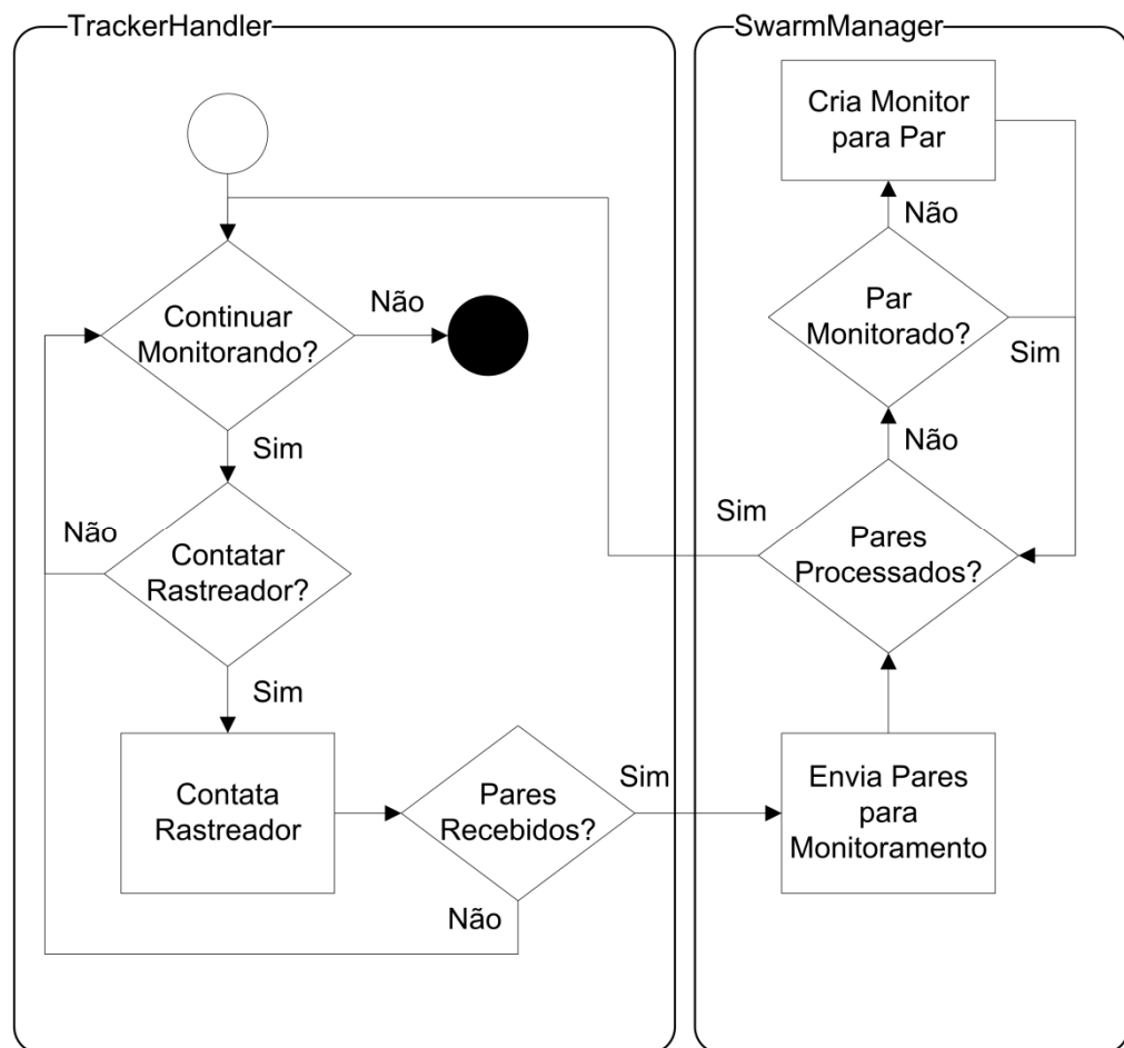
Figura 5.3: TrackerHandler
