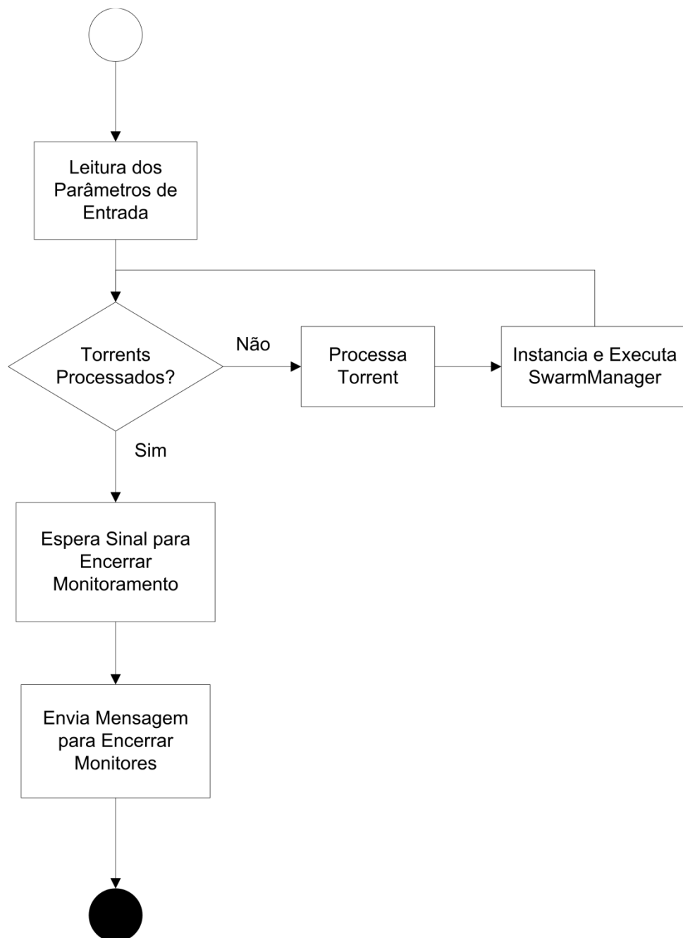
Figura 5.1: Global Manager
