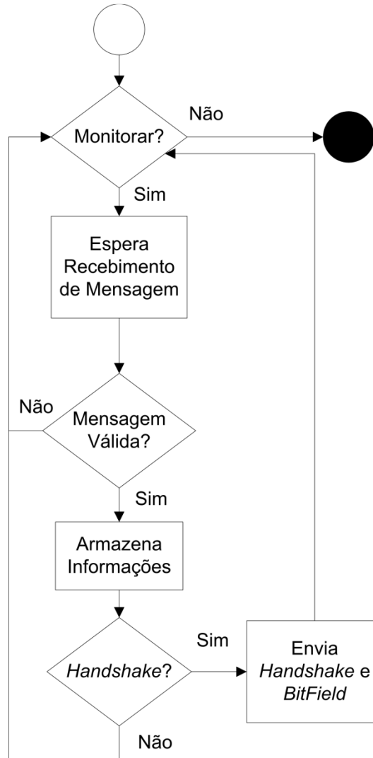
Figura 5.4: ActivePeerMonitor
