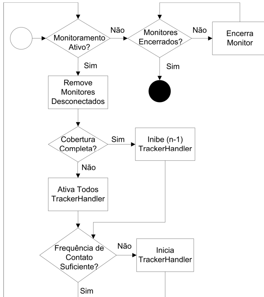
Figura 5.2: SwarmManager
