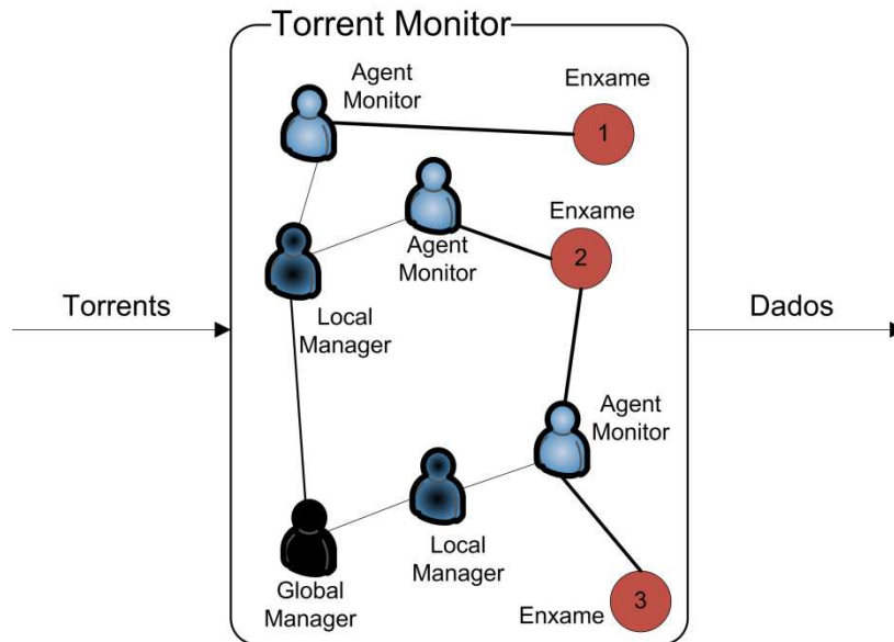
Figura 4.3: Subsistema Torrent Monitor
