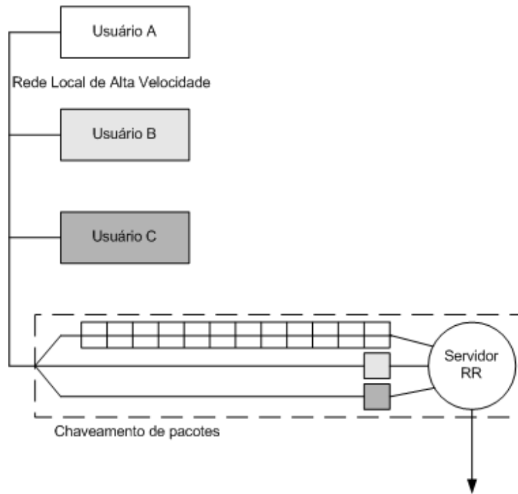
Figura 4.2: Servidor Round-Robin
