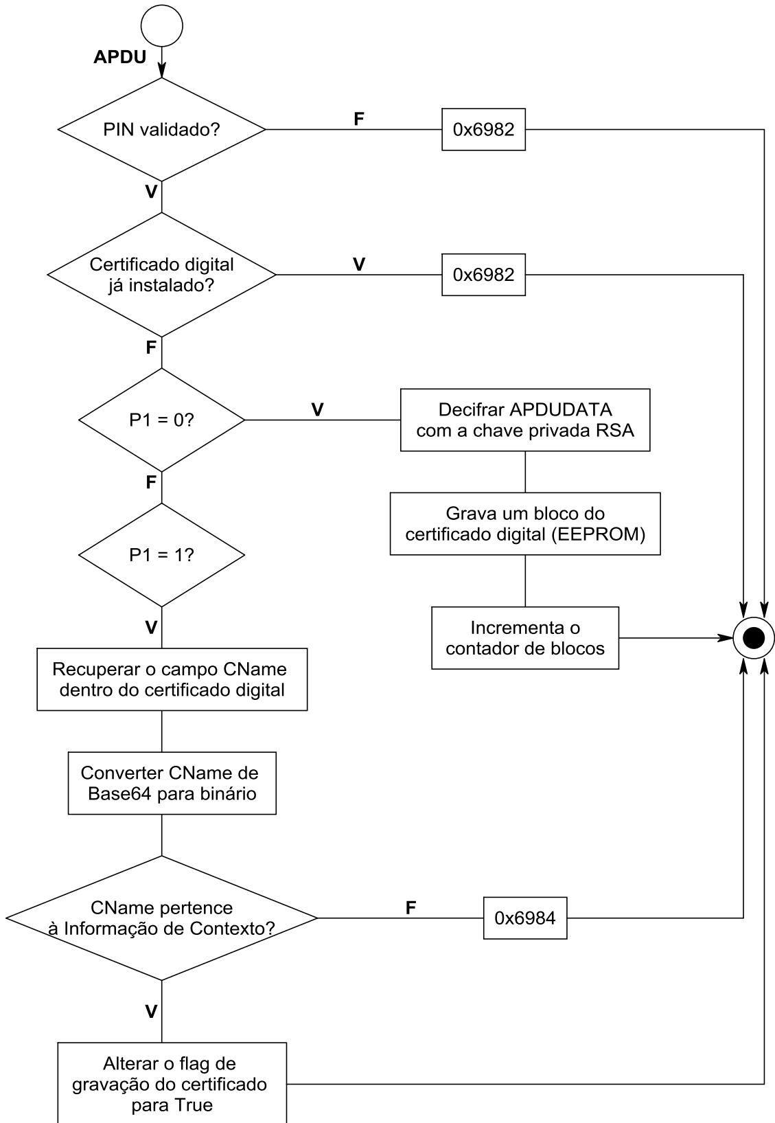
Gráfico 6-12 – Upload Certificado Digital
