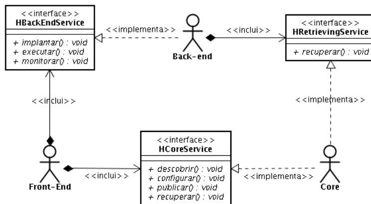
Figura 4.3: HCoreService
