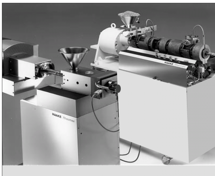
Figura 3.1 Extrusora dupla rosca Haake CTW100p Rheomex
