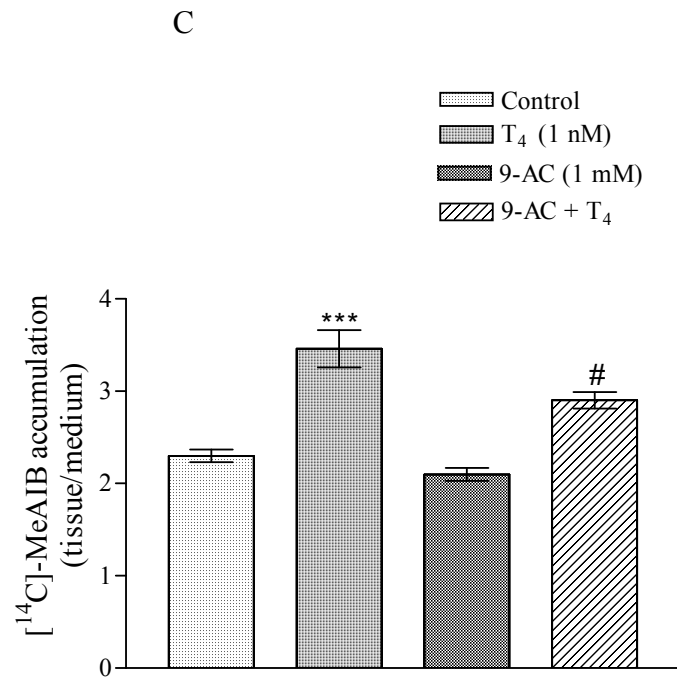
Figure 2. A) Effect of Apamine; B) Tolbutamide and C) 9-AC on the stimulatory action of T 4 on [ 14 C] MeAIB accumulation in rat testes. Means ± SEM for control. n = 4 for all groups. ***P < 0.001 compared with control; #p < 0.05; ###p < 0.001 compared with T 4 group. Pre-incubation time: 30 min; incubation time: 60 min.
