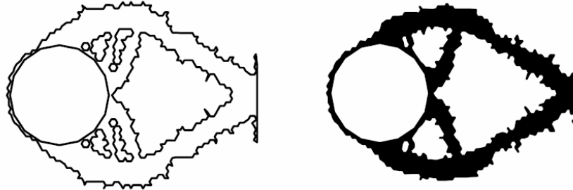
Figura 5.4.39 – Michell truss – usando MEC Marczak (2006)
