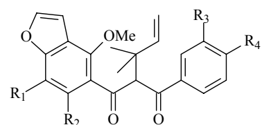
(44) R 1 = R 2 = R 3 = R 4 = H (45) R 1 + R 2 = OCH 2 O, R 3 = R 4 = H (46) R 1 = R 2 = OMe, R 3 = R 4 = H
