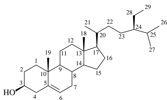
\beta -Sitosterol
