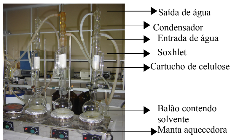
Figura 16. Extrator Soxhlet
