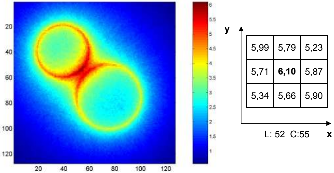
(b) GOS F(x,y) \text{ máx} = 6,105 \pm 0,126 \text{ MeV/g}
